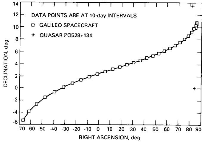
Fig. 1. Galileo EGA1 approach trajectory.
