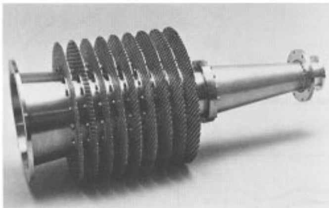
Fig. 5. Coolable dual-mode feedhorn.
