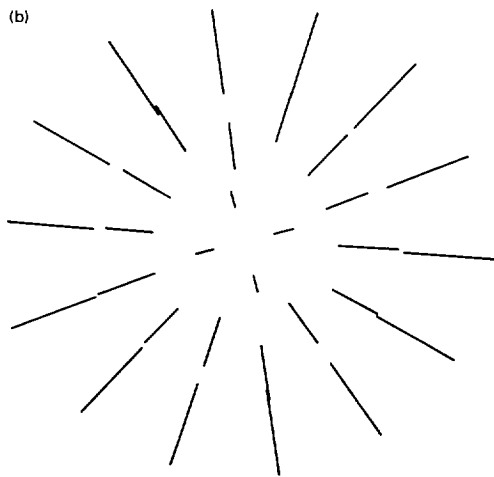
Fig. 3. Comparison of rf-trapped macroparticles with simulation: (a) photograph from [4] showing the "crystalline" state of 32 particles, and (b) results from the simulation of 32 trapped particles.
