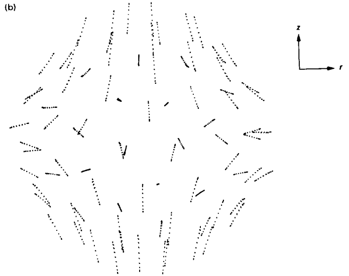
Fig. 4. Comparison of \approx 100 rf-trapped particles with simulation: (a) photograph from [4] showing \approx 100 particles outlining the fields in the trap, and (b) results from the simulation of 128 rf-trapped particles.
