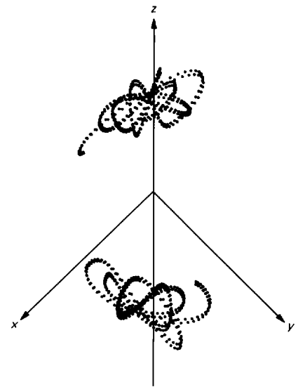
Fig. 7. The system of Fig. 6, after much of the precessional motion has damped out, sits stably along the z-axis.
