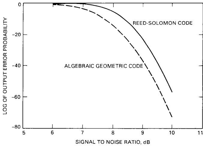
Fig. 1. Comparison of algebraic geometric code C(1) and Reed-Solomon code (511, 127).
