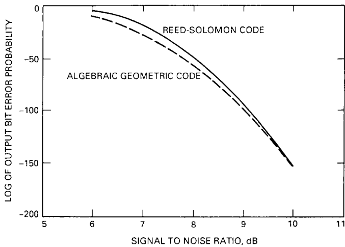
Fig. 2. Comparison of algebraic geometric code C(2) and Reed-Solomon code (511, 255).
