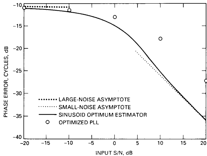
Fig. 2. Phase-error performance of an optimized phase-locked loop subject to the same signal-to-noise ratio and observation interval as the optimum estimator.
