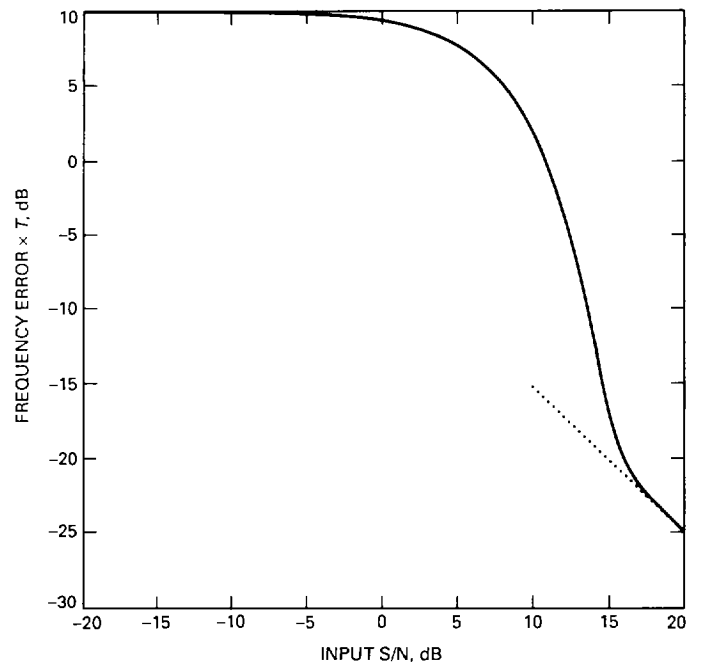
Fig. 4. Frequency error performance of the optimum estimator for the case of unknown constant frequency. The small-noise asymptote comes from Eq. (99) of [2]. The large-noise asymptote (not plotted) is at 10.04 dB. This corresponds to a frequency error uniformly distributed from -5.5/T to +5.5/T .
