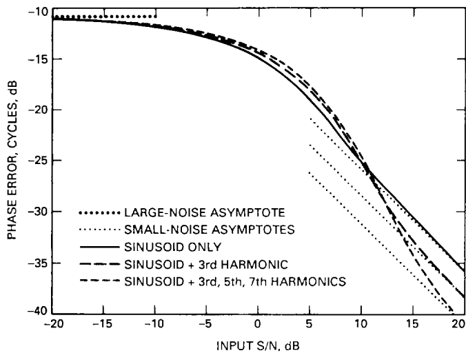
Fig. 1. Phase-error performance of three optimum estimation algorithms for the case of known constant frequency. The large-noise asymptote corresponds to phase error uniformly distributed over one cycle. The three small-noise asymptotes come from Eqs. (54), (59), and a similar equation for the first four components of a square wave, obtained by using Eq. (56) of [1].
