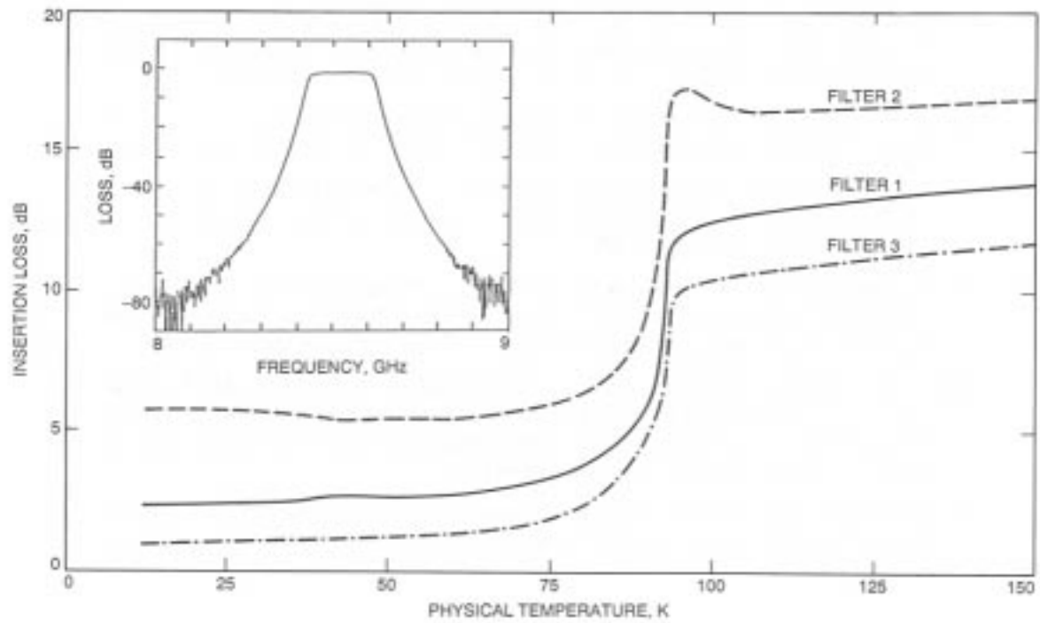
Fig. 2. Insertion loss ( L_s ) versus physical temperature ( T ) for three separate filters. The measurements were taken at an input power of 38 \mu\text{W} .
