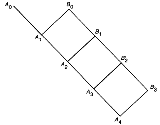
Fig. 3. The subspaces needed for the construction of a noncatastrophic encoder for the [24, 12, 10, 16] code.
