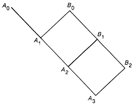
Fig. 2. The subspaces needed for the construction of a noncatastrophic encoder for the [24, 12, 7, 12] PUM code.
