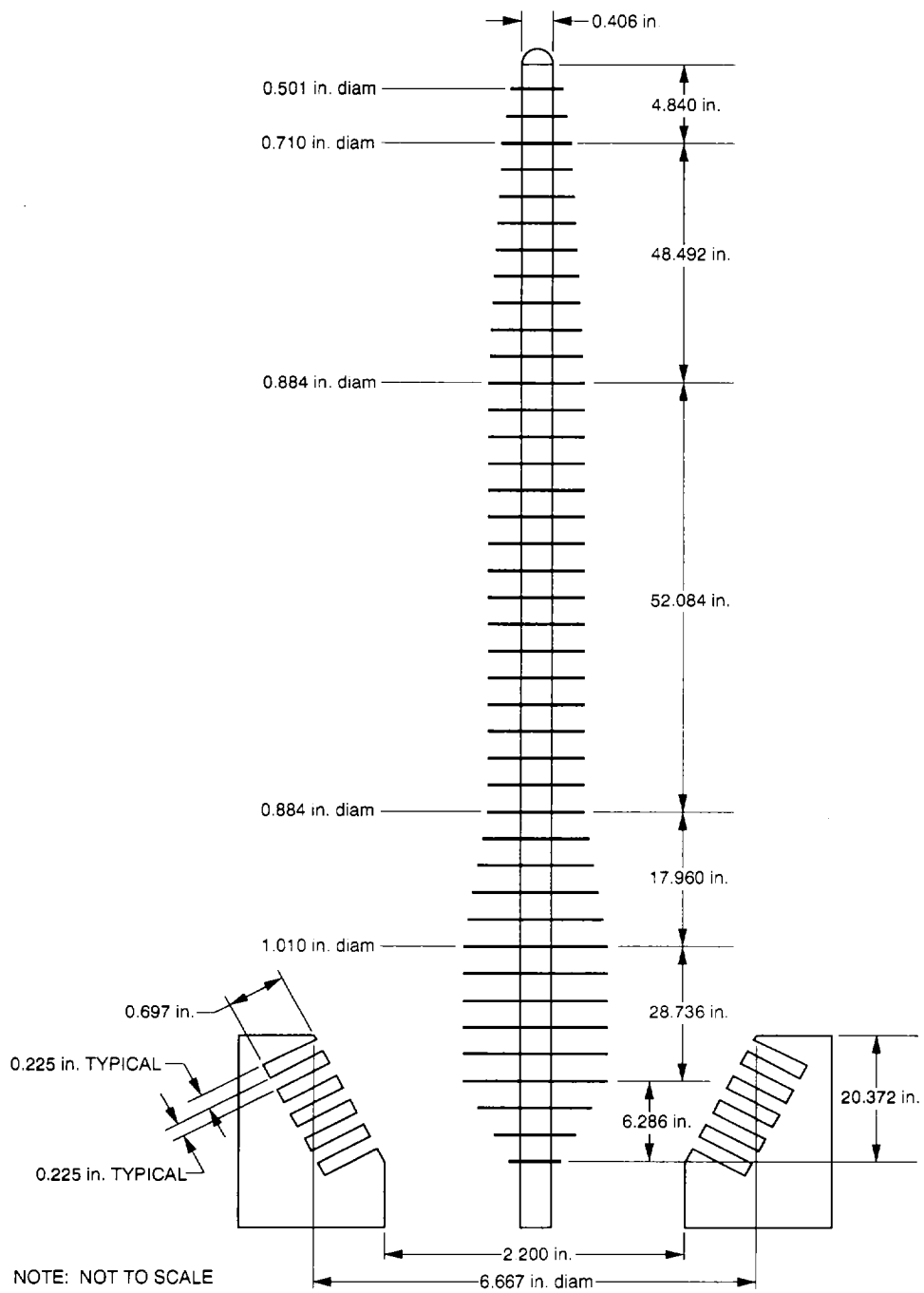
Fig. 3. C-band disc-on-rod and launching horn.
