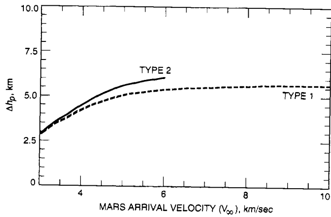
Fig. 13. Three-sigma altitude uncertainty versus Mars arrival velocity (DSN Doppler/dual-spacecraft VLBI).
