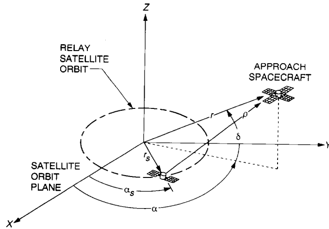
Fig. 7. Spacecraft-spacecraft tracking geometry.
