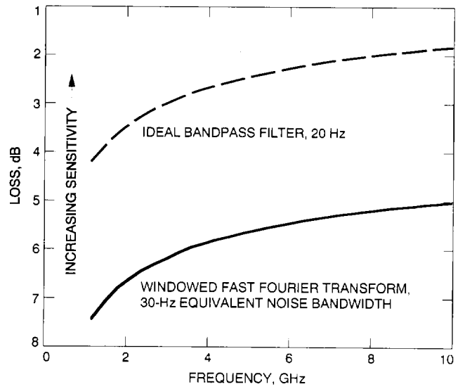
Fig. 3. A comparison of losses relative to the theoretical optimum.
