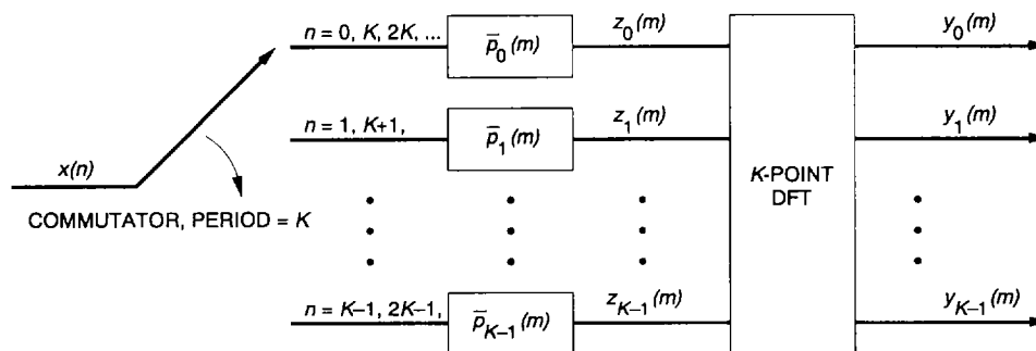
Fig. 7. Discrete Fourier transform implementation for a bank of identically spaced, identically shaped filters.
