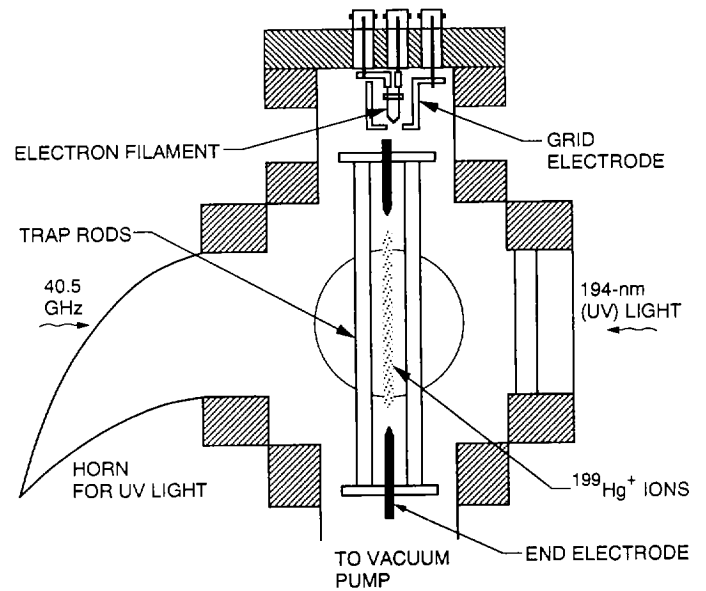
Fig. 2. Linear ion trap assembly residing in its high vacuum enclosure. State selection light from the ^{202}\text{Hg} discharge lamp enters from the right, is focused onto the central 1/3 of the trap and is collected in the horn. Fluorescence from the trapped ions is collected in a direction normal to the page.
