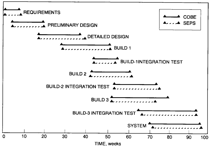
Fig. 22. Schedule comparison.
