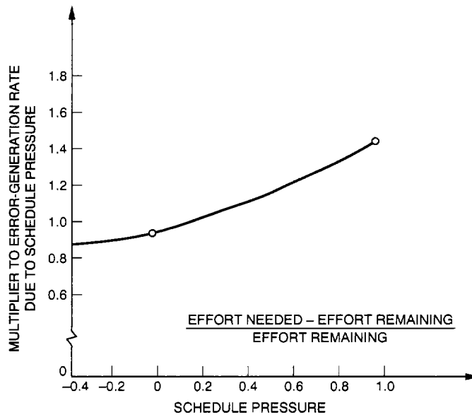
Fig. 7. Schedule pressure factor on error-generation rate.
