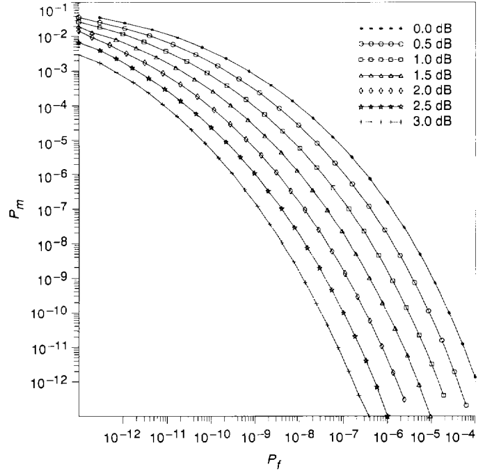
Fig. 3. P_m versus P_f for the (15,1/4) code ( J = 4 ).
