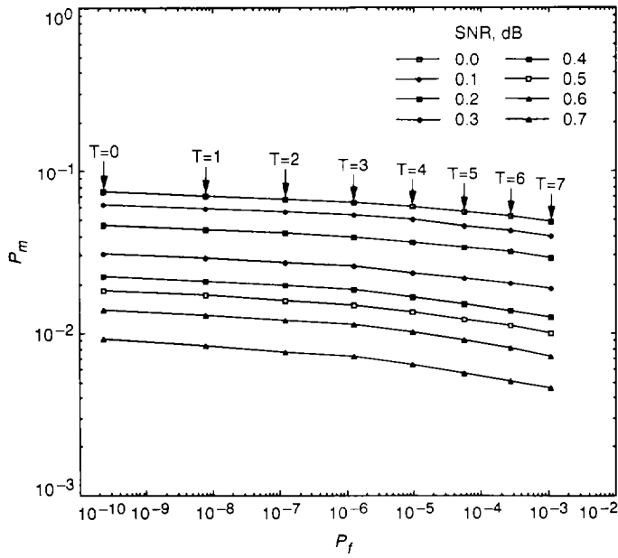
Fig. 1. P_m versus P_f (frame length = 8960 bits).
