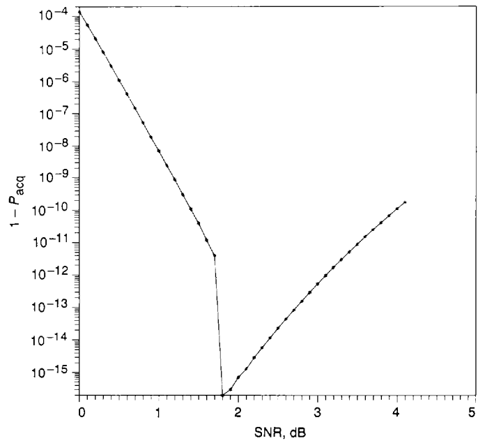
Fig. 9. (15,1/4) code-acquisition performance of scheme 3 using a fixed threshold from 0–4 dB (64-bit sync marker).
