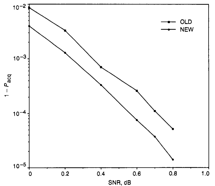
Fig. 8. P_{acq} of the old and new strategies.
