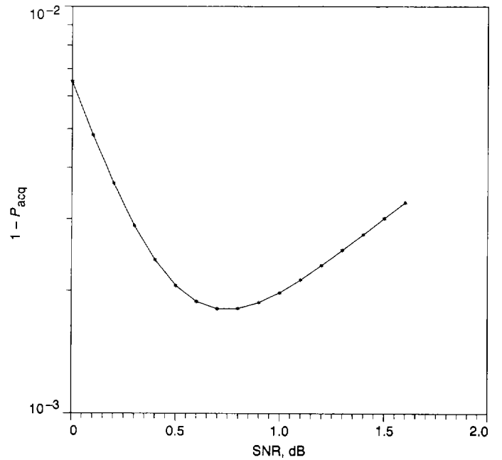
Fig. 7. (15,1/4) code-acquisition performance of scheme 3 using a fixed threshold from 0–1.5 dB.
