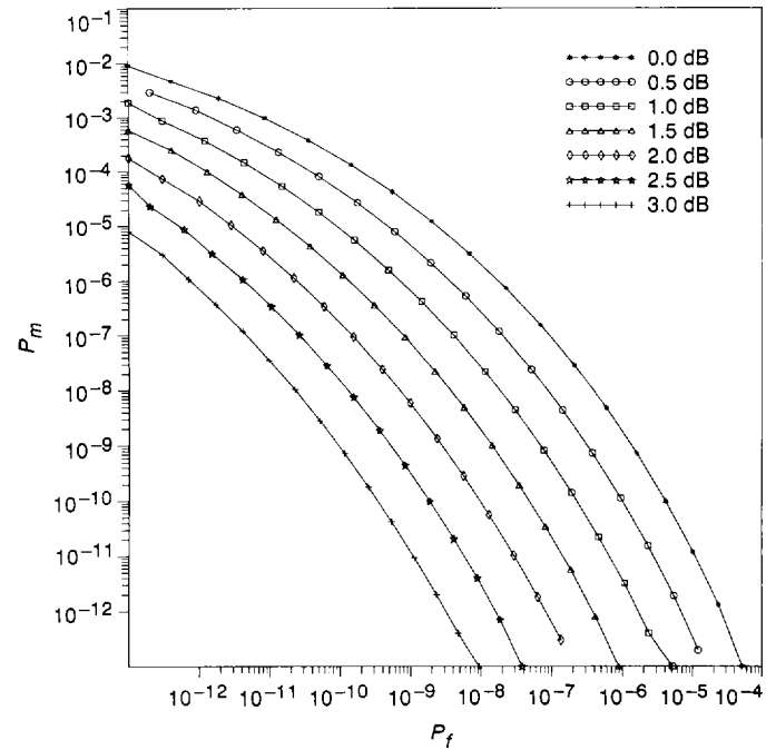
Fig. 4. P_m versus P_f for the (15,1/6) code ( J = 4 ).
