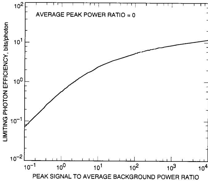
Fig. 1. Photon efficiency versus peak signal to average background power ratio in the limit of average power to peak power ratio equals 0 (i.e., with extremely low duty cycle).
