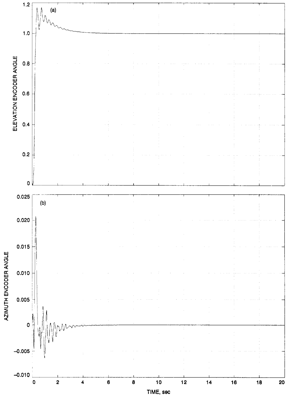
Fig. 20. Closed-loop response to step input for proportional weight 100 and integral weight 70 (both in azimuth and elevation), and weights for the flexible subsystem equal to 1 \times 10^{-7} : (a) elevation encoder angle to elevation step command; (b) azimuth encoder angle to elevation step command; (c) azimuth encoder angle to azimuth step command; and (d) elevation encoder angle to azimuth step command.
