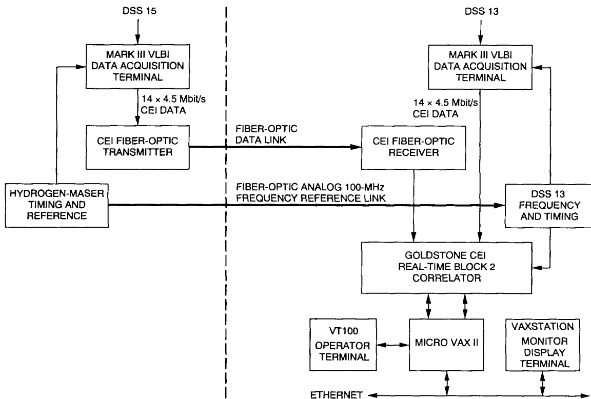
Fig. 4. Goldstone real-time CEI block diagram.
