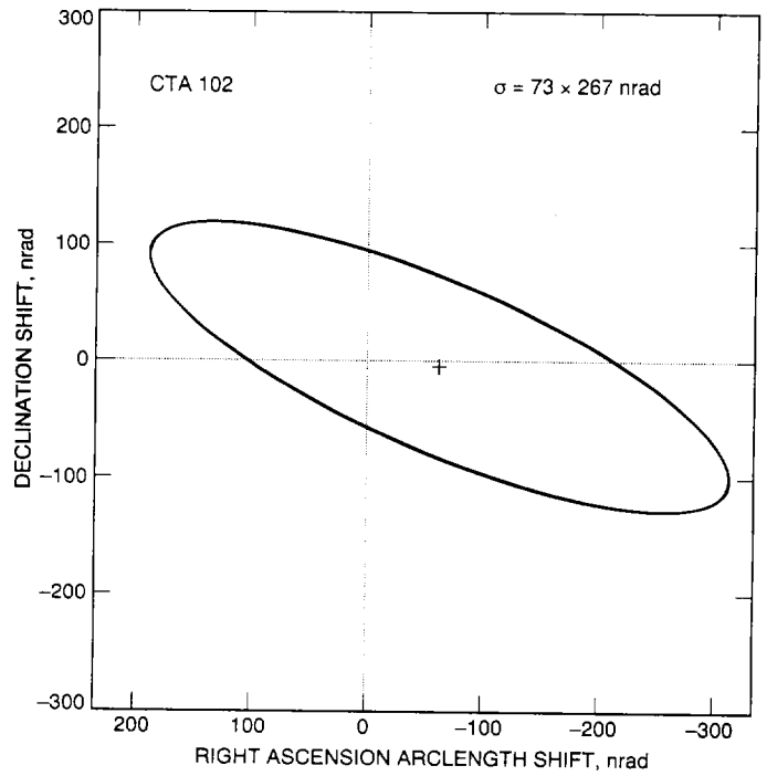
Fig. 3. Angular accuracy achieved for a non-real-time phase delay experiment on the 21-km DSS-13–DSS-15 baseline.
