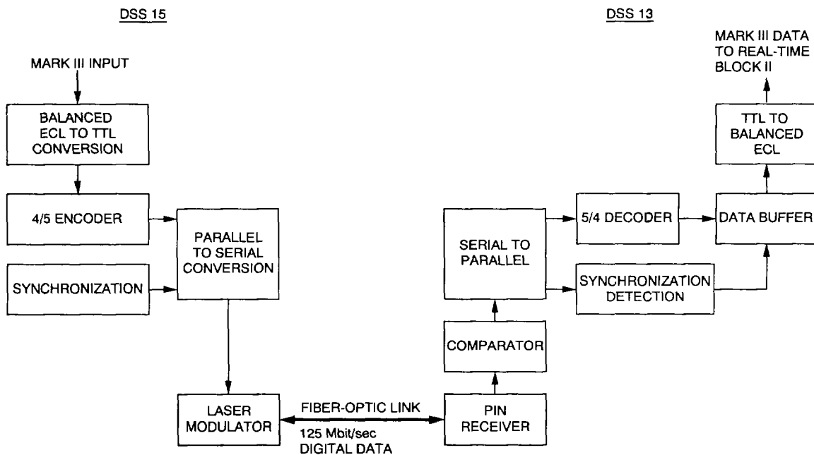
Fig. 5. Fiber-optic digital data link block diagram.
