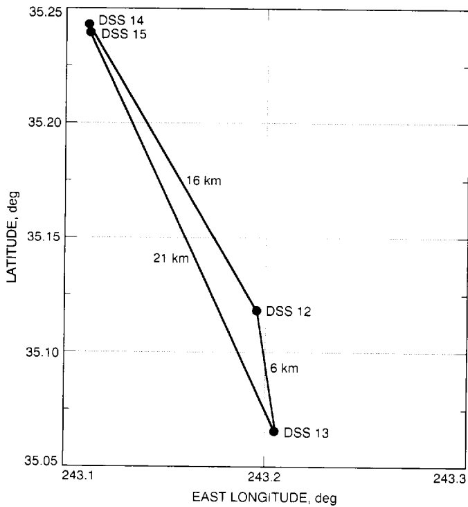
Fig. 2. Existing antennas and CEI baselines at the Goldstone DSCC.
