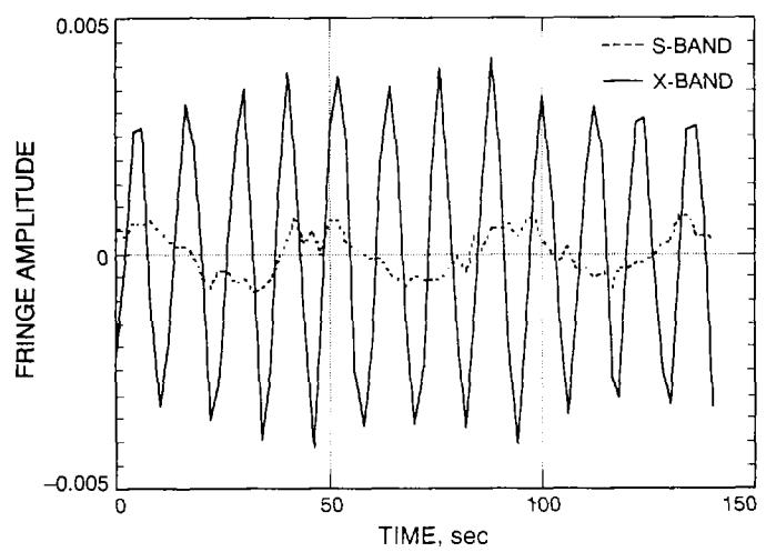
Fig. 7. First real-time fringes obtained on the Goldstone real-time CEI.
