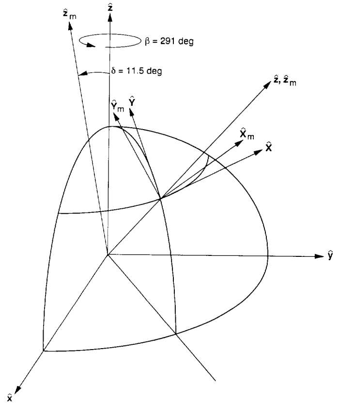
Fig. 3. A graphical illustration of all the frames used in the text. The vectors \hat{x} , \hat{y} , and \hat{z} correspond to the geodetic frame; the vectors \hat{x}_m , \hat{y}_m , and \hat{z}_m correspond to the geomagnetic frame; the vectors \hat{X}_m , \hat{Y}_m , and \hat{Z}_m correspond to geodetic local east, north, and vertical; and the vectors \hat{X}_m , \hat{Y}_m , and \hat{Z}_m correspond to geomagnetic local east, north, and vertical.
