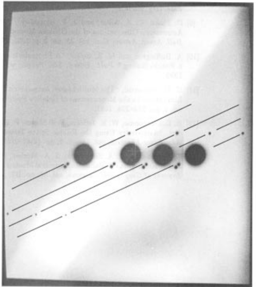
Fig. 2. NOFS multiplexed CCD picture of Jupiter's Galilean satellites (courtesy of D. G. Monet, NOFS).
