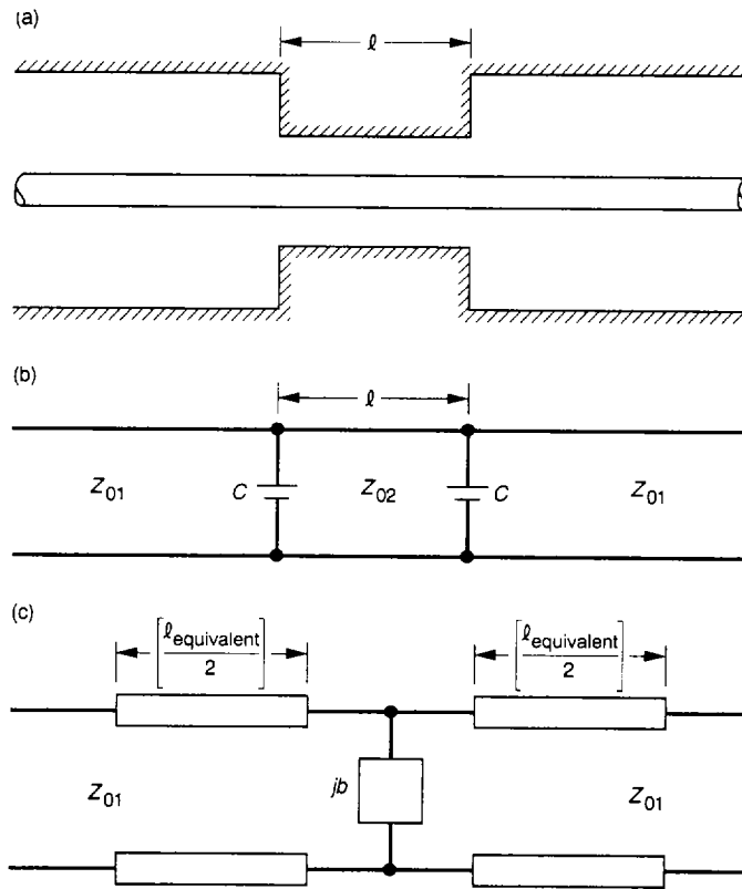
Fig. C-1. Cable with a section of reduced outer diameter: (a) physical representation; (b) equivalent circuit with two capacitive shunt discontinuities separated by a line length of reduced section; and (c) equivalent circuit with a single shunt discontinuity and equivalent line lengths.
