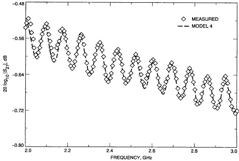
Fig. 13. Comparison of theoretical and measured insertion losses for Model 4 for the pre-environmental cable condition.
