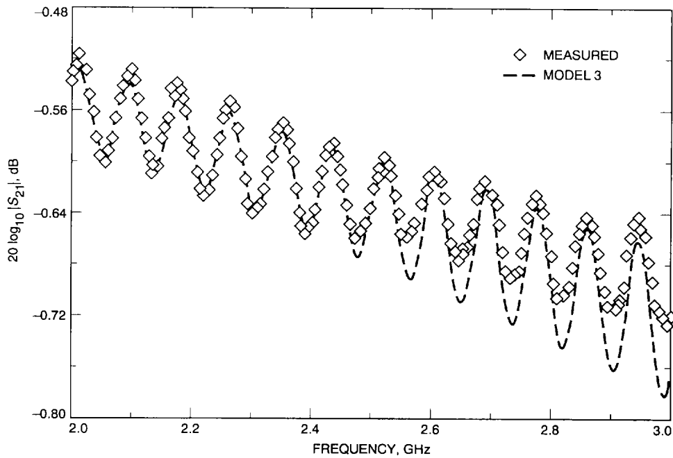
Fig. 8. Comparison of theoretical and measured insertion losses for Model 3 for the pre-environmental cable condition.
