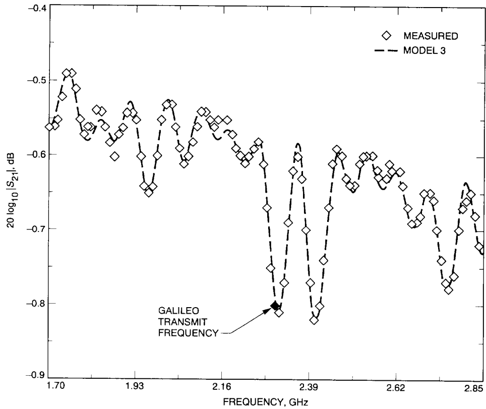
Fig. 7. Comparison of theoretical and measured insertion losses for Model 3, assuming shunt capacitance values that are constant over the frequency range of interest.
