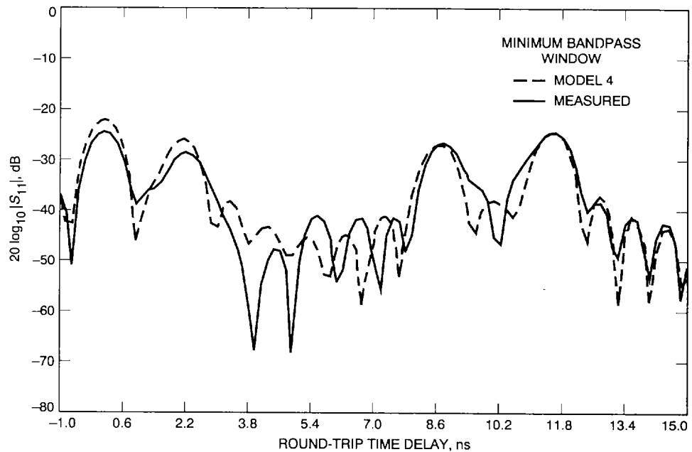
Fig. 15. Comparison of theoretical and measured time domain responses based on |S_{11}| data for Model 4. The theoretical response curve had to be moved by the equivalent of 1.081 in. (0.212 nsec, round-trip) to the left in order to line up the peaks of curves.
