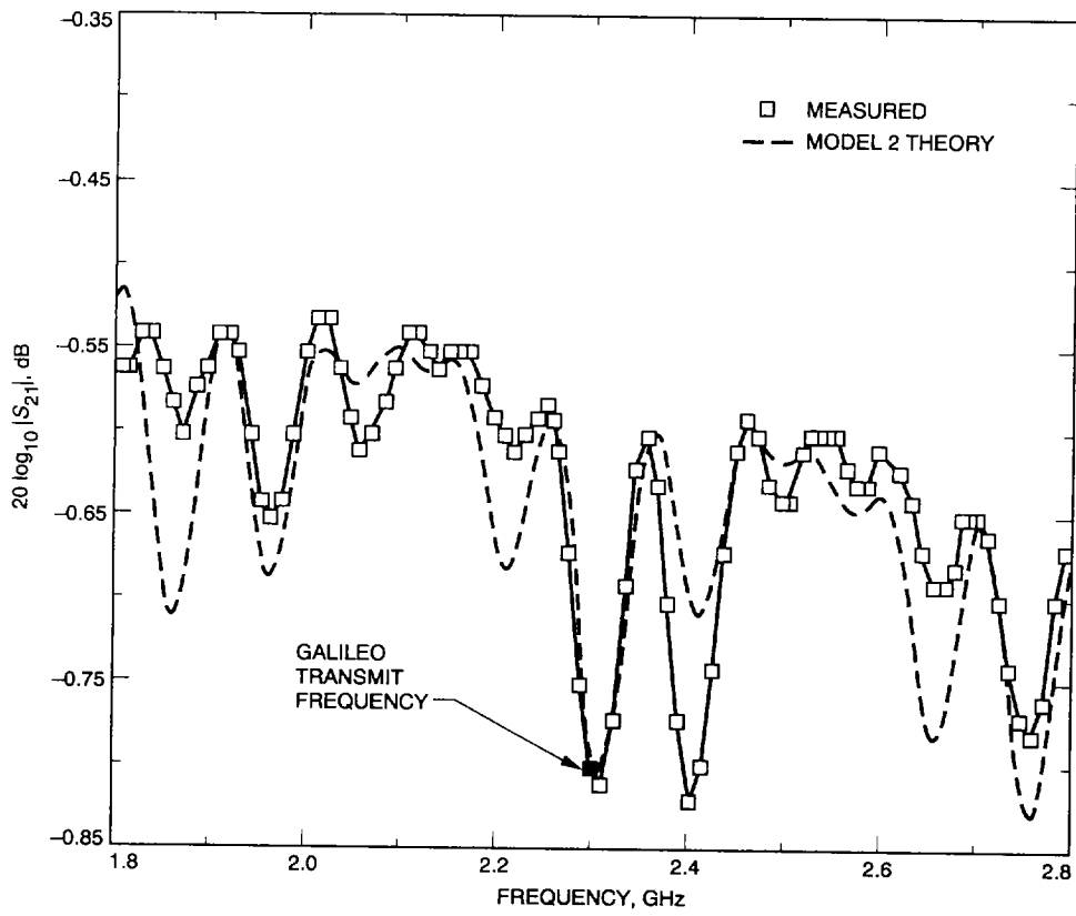
Fig. 1. Comparison of experimental and Model 2 theoretical data.
