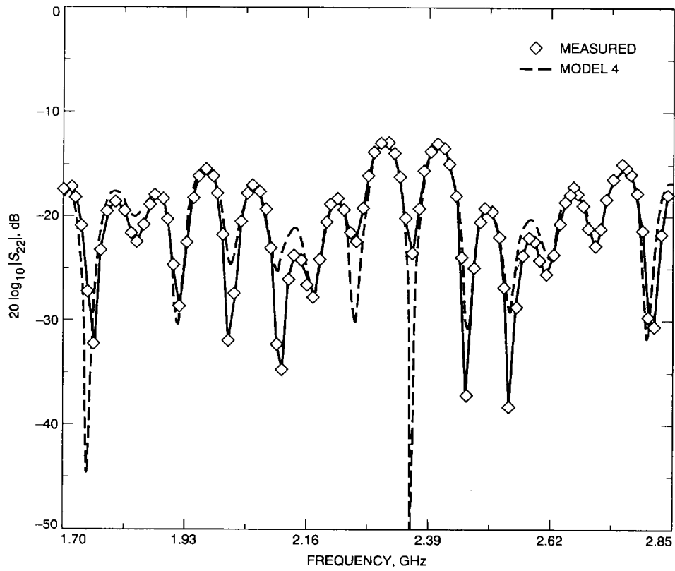
Fig. 12. Comparison of theoretical and measured return losses for Model 4, as seen looking into port 2.
