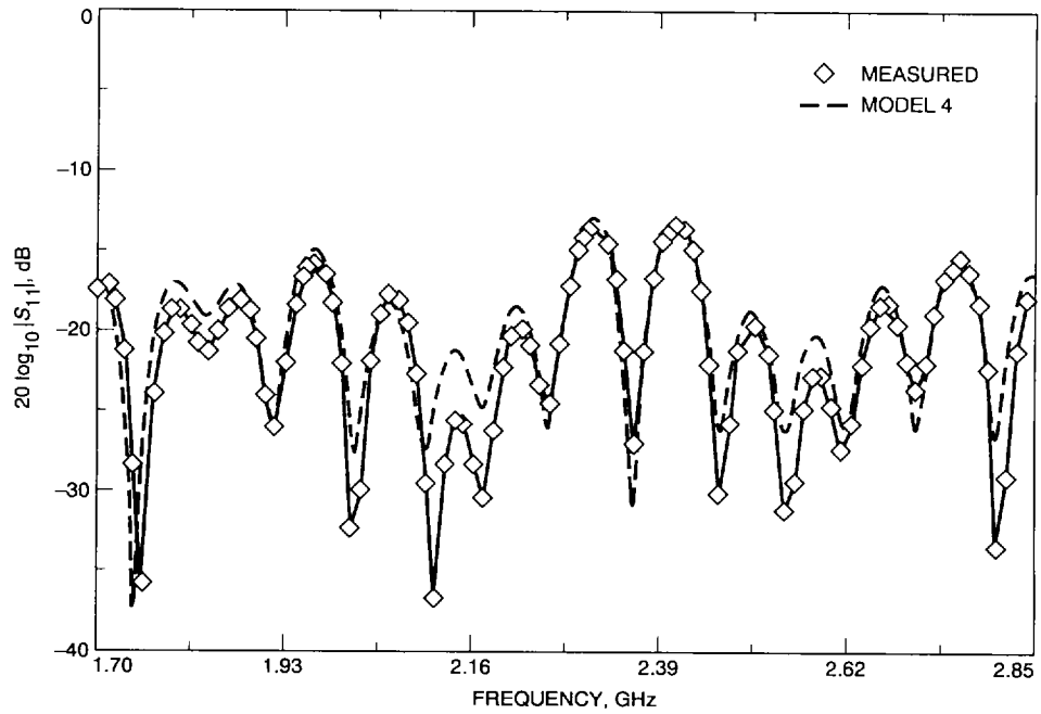
Fig. 11. Comparison of theoretical and measured return losses for Model 4, as seen looking into port 1.
