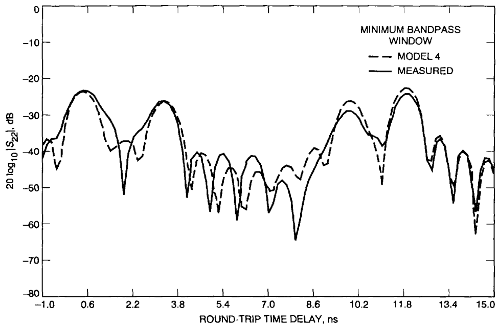
Fig. 16. Comparison of theoretical and measured time domain responses based on |S_{22}| data for Model 4. The theoretical response curve had to be moved by the equivalent of 1.376 in. (0.270 nsec, round-trip) to the right in order to line up the peaks of curves.
