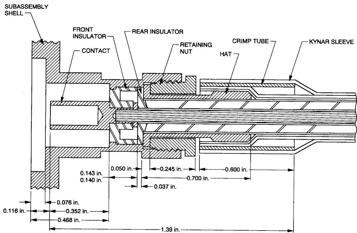
Fig. 5. Connector details.
