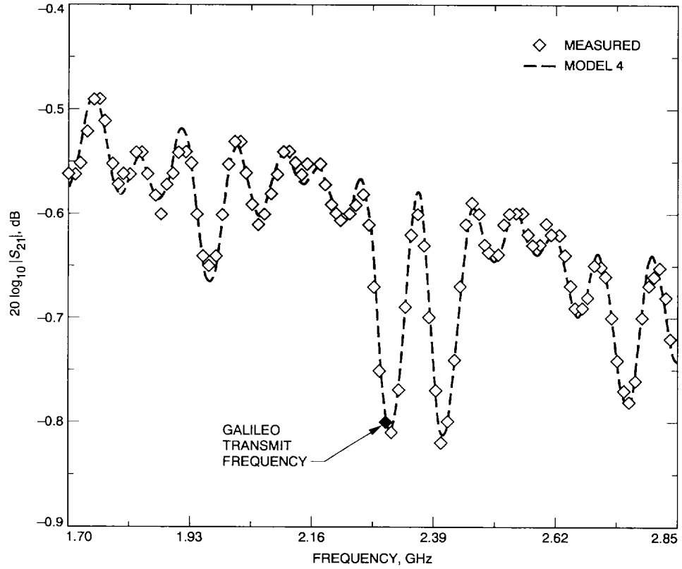
Fig. 10. Comparison of theoretical and measured Insertion losses for Model 4, assuming capacitive shunt susceptance values that are constant over the frequency range of interest.
