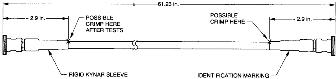
Fig. 4. Galileo S-band cable outer dimension detail.
