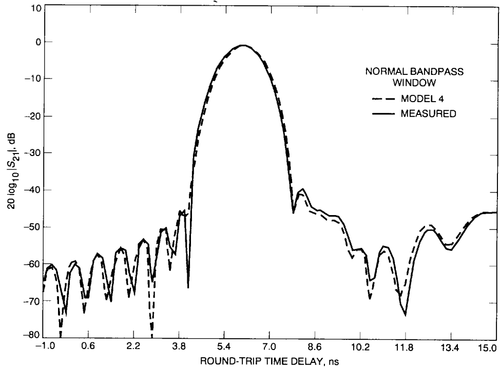
Fig. 14. Comparison of theoretical and measured time domain responses on |S_{21}| data for Model 4.
