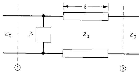
Fig. A-1. Basic network used in cable model.
