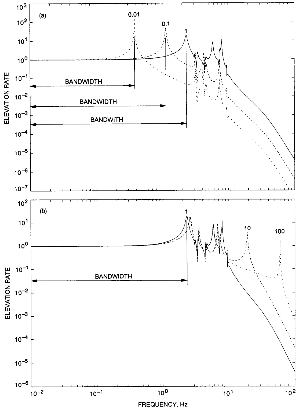
Fig. 5. Transfer functions: elevation rate output to elevation rate command.
