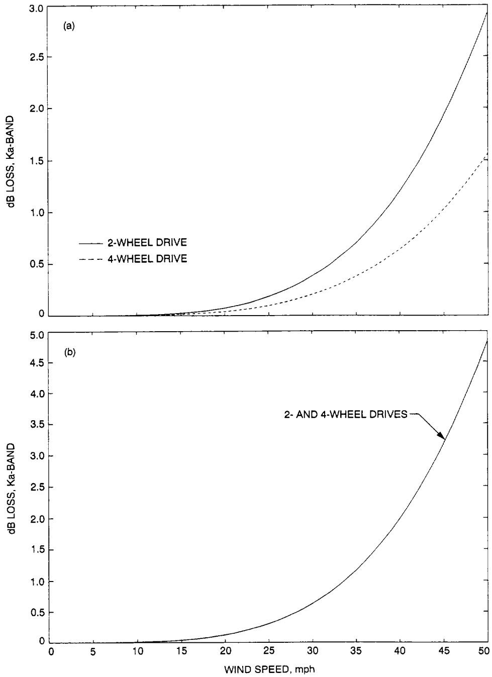
Fig. 10. Ka-band decibel loss due to wind gusts: (a) x-direction wind and (b) y-direction wind.
