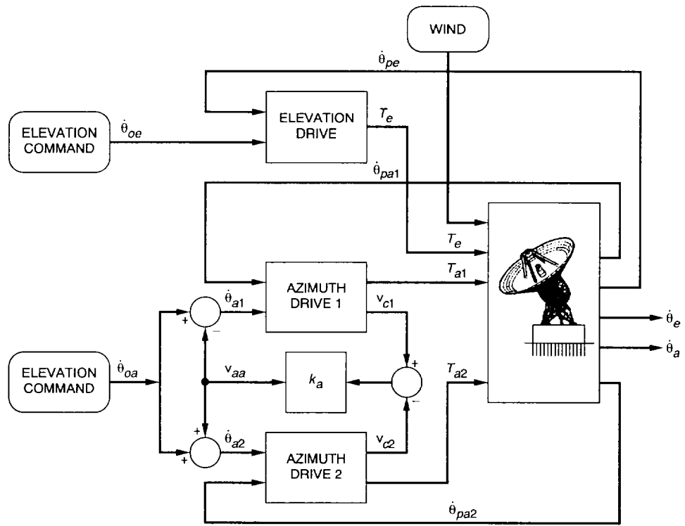
Fig. 3. Rate-loop model of the antenna.
