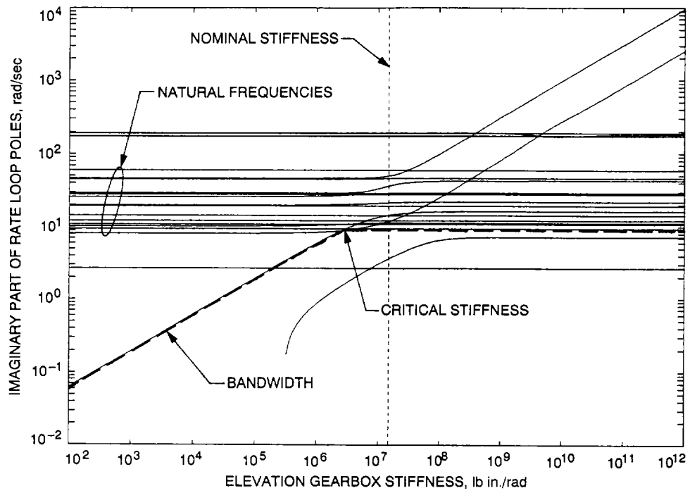
Fig. 4. Imaginary parts of the rate-loop poles versus elevation gearbox stiffness.
