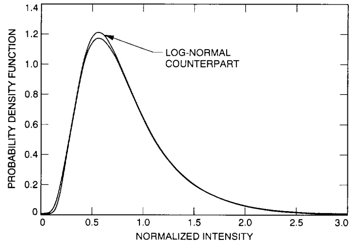
Fig. 8. Probability density function of the normalized intensity, \beta = 5 and \sigma_\ell = 0.5 , and its approximated log-normal counterpart.
