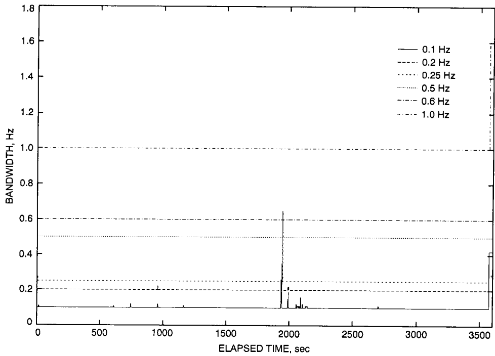
Fig. 8. Loop bandwidth for Galileo carrier phase recovery at various B_0 . The events near \sim 3570 sec are due to a switch from one-way to two-way tracking.
