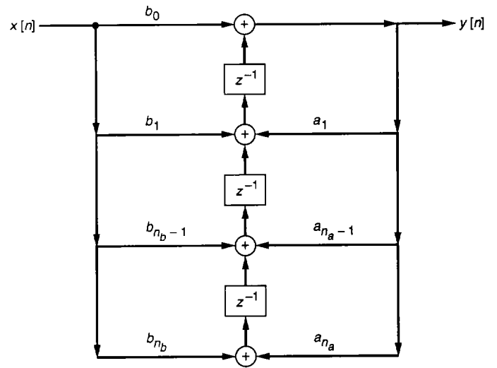
Fig. 6. Direct form 2 transposed filter structure.
