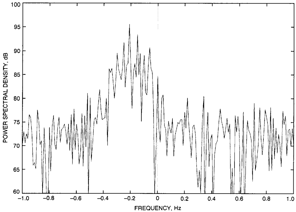
Fig. 3. Observed typical power spectrum (at baseband) for the Pioneer 10 carrier.
