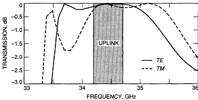
Fig. 4. Transmission coefficient versus frequency for Ka-/Ka-band dichroic plate with stepped rectangular apertures for TE and TM polarizations at Ka-band uplink.
