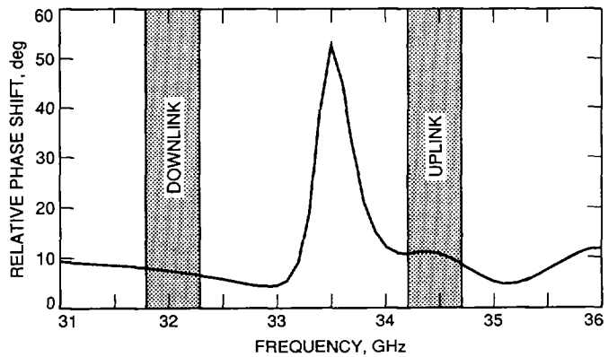
Fig. 5. Relative phase shift versus frequency for Ka-/Ka-band dichroic plate with stepped rectangular apertures.
