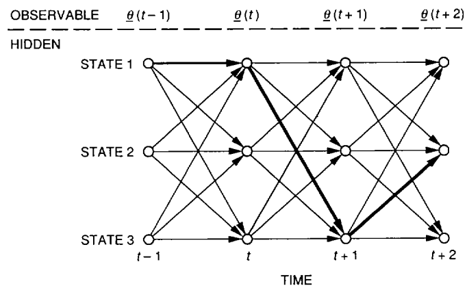
Fig. A-1. An illustrative example of a three-state hidden Markov model.
