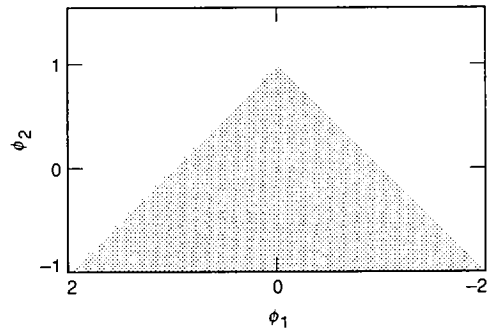
Fig. 1. Admissible region for AR(2) parameters.
