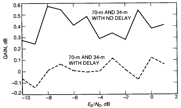
Fig. 7. Gain over the 70-m antenna.
