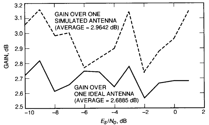
Fig. 3. Gain from combining two identical antennas.
