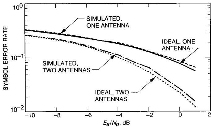
Fig. 2. Combining two identical antennas.
