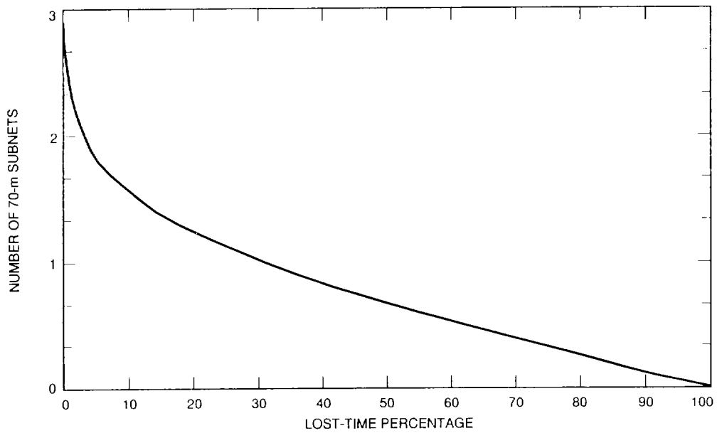
Fig. 6. Resources-versus-lost-time graph for the 70-m subnet in 1995.
