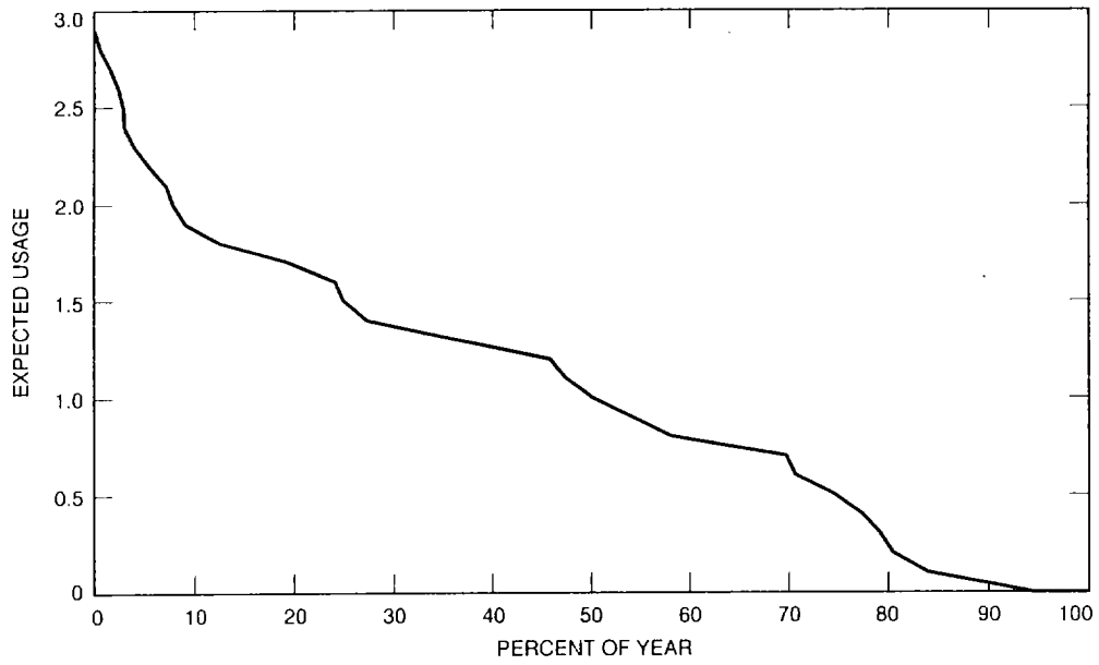
Fig. 5. Load-duration curve for the 70-m subnet in 1995.
