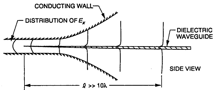
Fig. A-2. Transverse electric field transition from an enclosed guide to an open dielectric ribbon guide.
