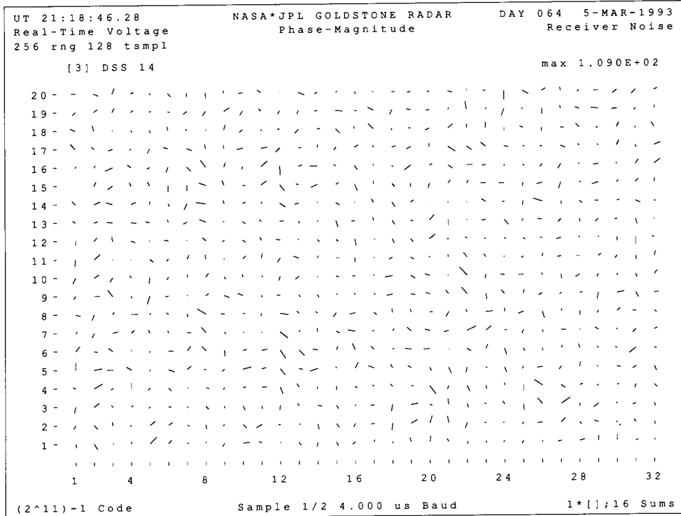
Fig. 3. Gaussian noise.
