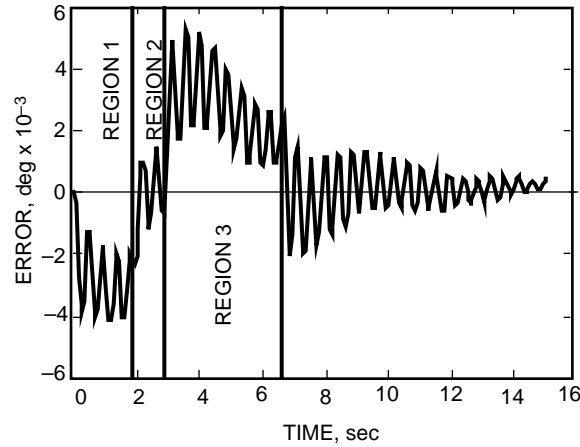
Fig. 4. Anticipated servo error for Example (1) with constant acceleration in regions 1 and 3 (elevation only).
