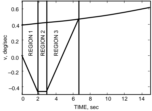
Fig. 2. Matching of antenna and target velocities for constant accelerations (elevation only).
