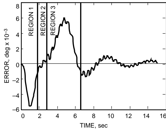
Fig. 8. Anticipated servo error (for Example (1) with raised cosine acceleration in regions 1 and 2 (elevation only)).
