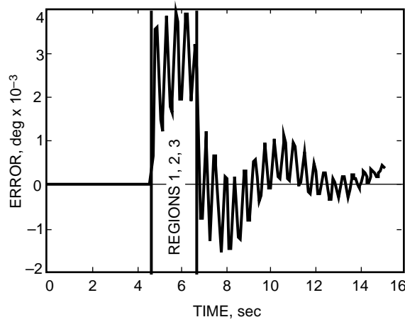
Fig. 9. Anticipated servo error during acquisition for Example (2), ( t_3 = 0.1 sec, t_2 = 0 ) (elevation only).
