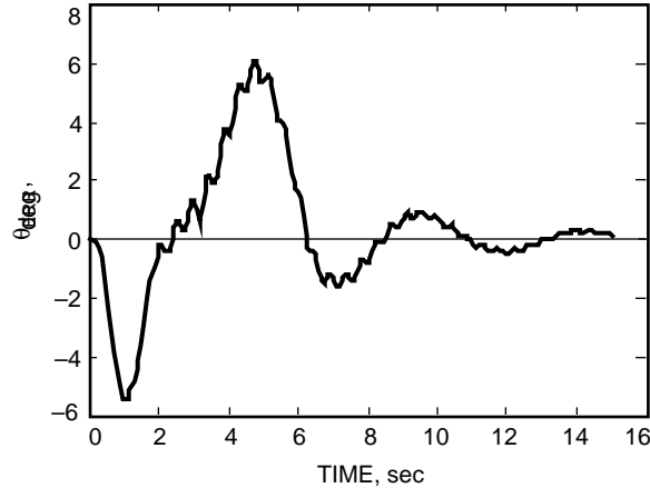
Fig. 10. Servo error for acquisition scheme 3 and constant velocity track. Acquisition is at t = 6.6 sec.
