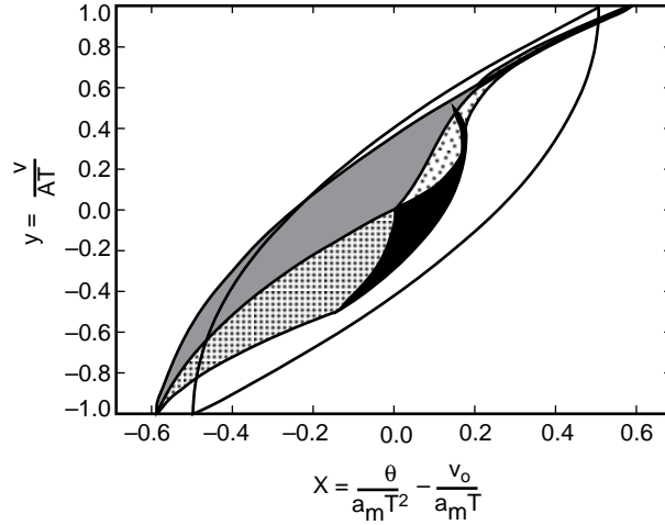
Fig. 11. Shrinkage of region of valid solutions for a_f = -a_0 = a_m .
