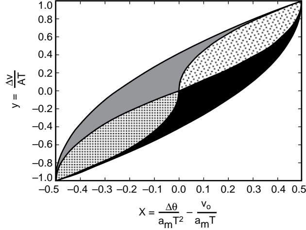
Fig. 5. Area of valid solutions ( a_m = a_{max}/2 and a_0 = a_f = 0 ).
