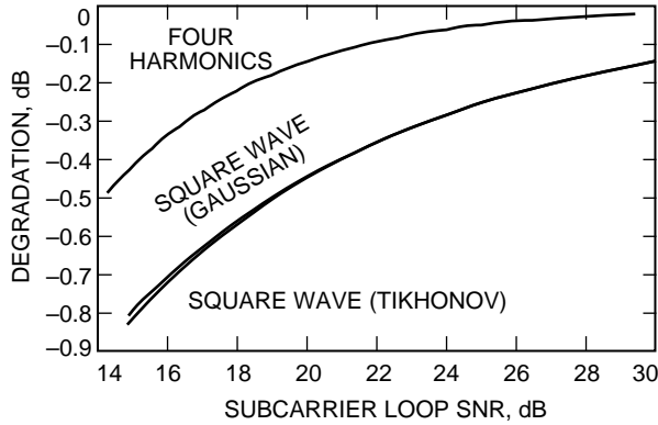
Fig. 1. Degradation due to the subcarrier loop versus loop SNR.
