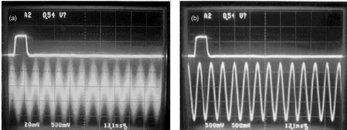
Fig. 9. Carrier recovery measurement in the time domain: (a) spoiled carrier and (b) recovered carrier.
