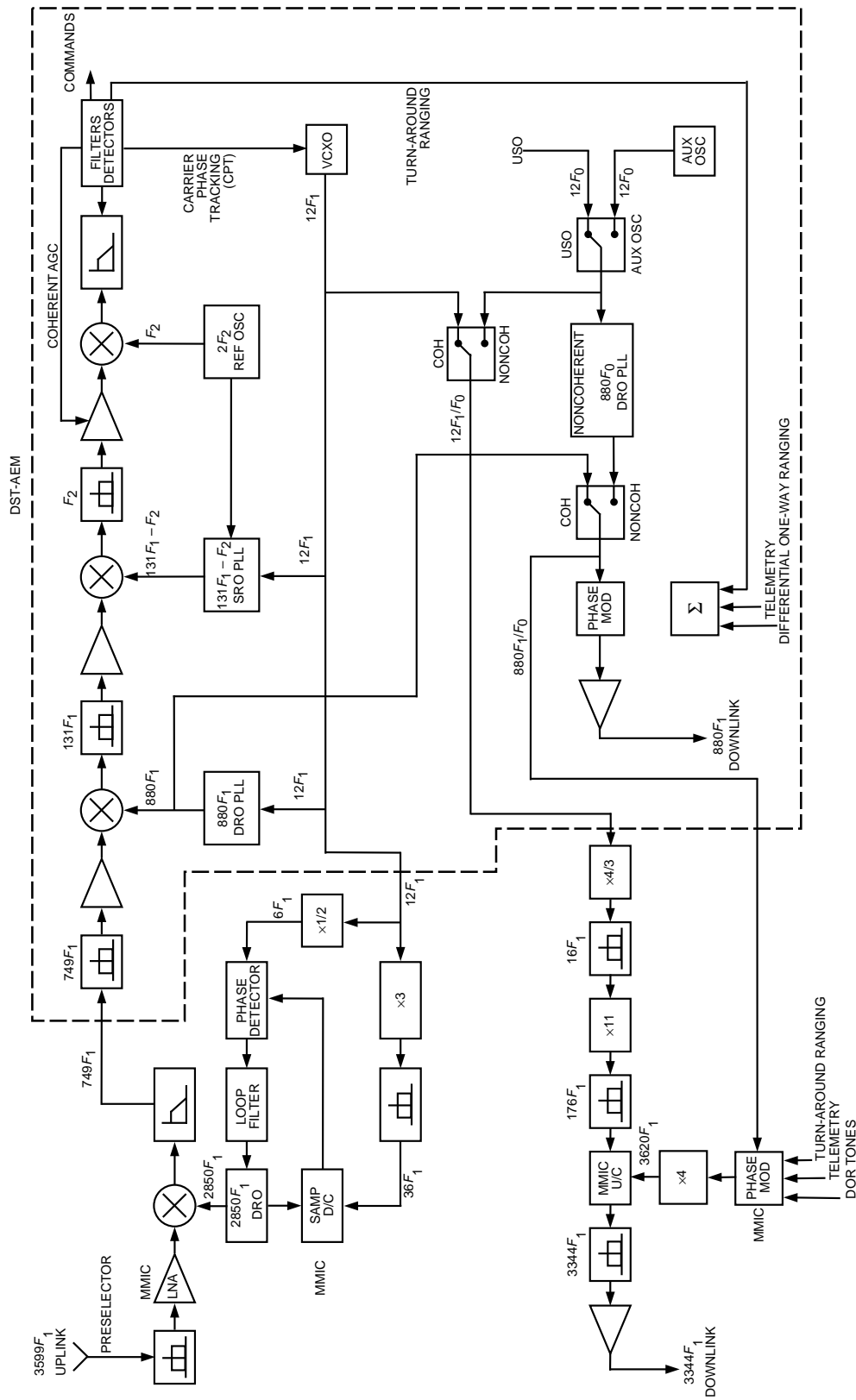
Fig. 1. Ka-band transponder functional block diagram.
