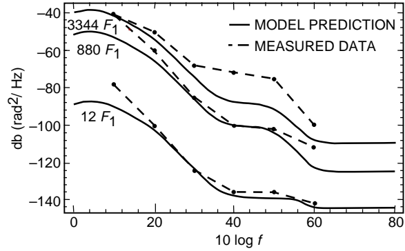
Fig. 5. Comparison of theoretical and measured coherent-mode phase noise densities (uplink = -100 dBm).
