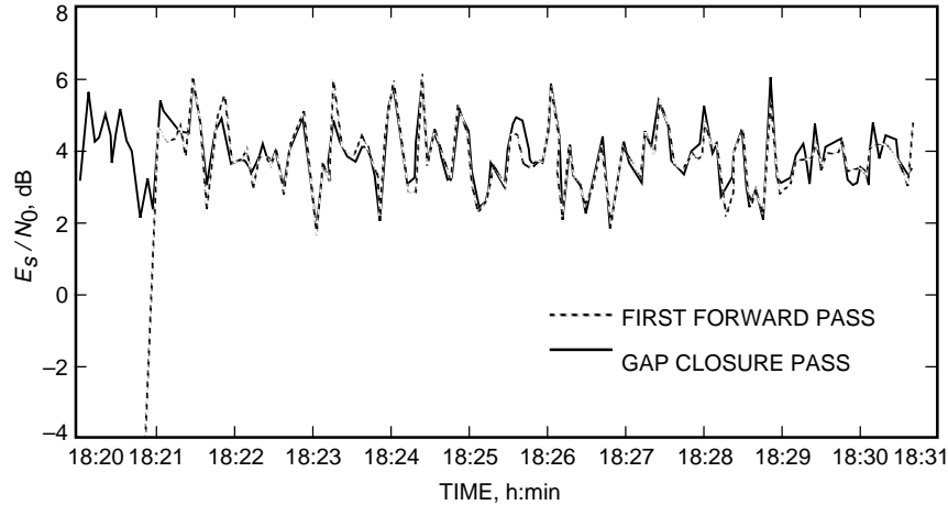
Fig. 5. The estimated symbol SNR versus time.
