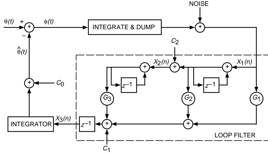
Fig. 2. Augmented third-order digital phase-locked loop.
