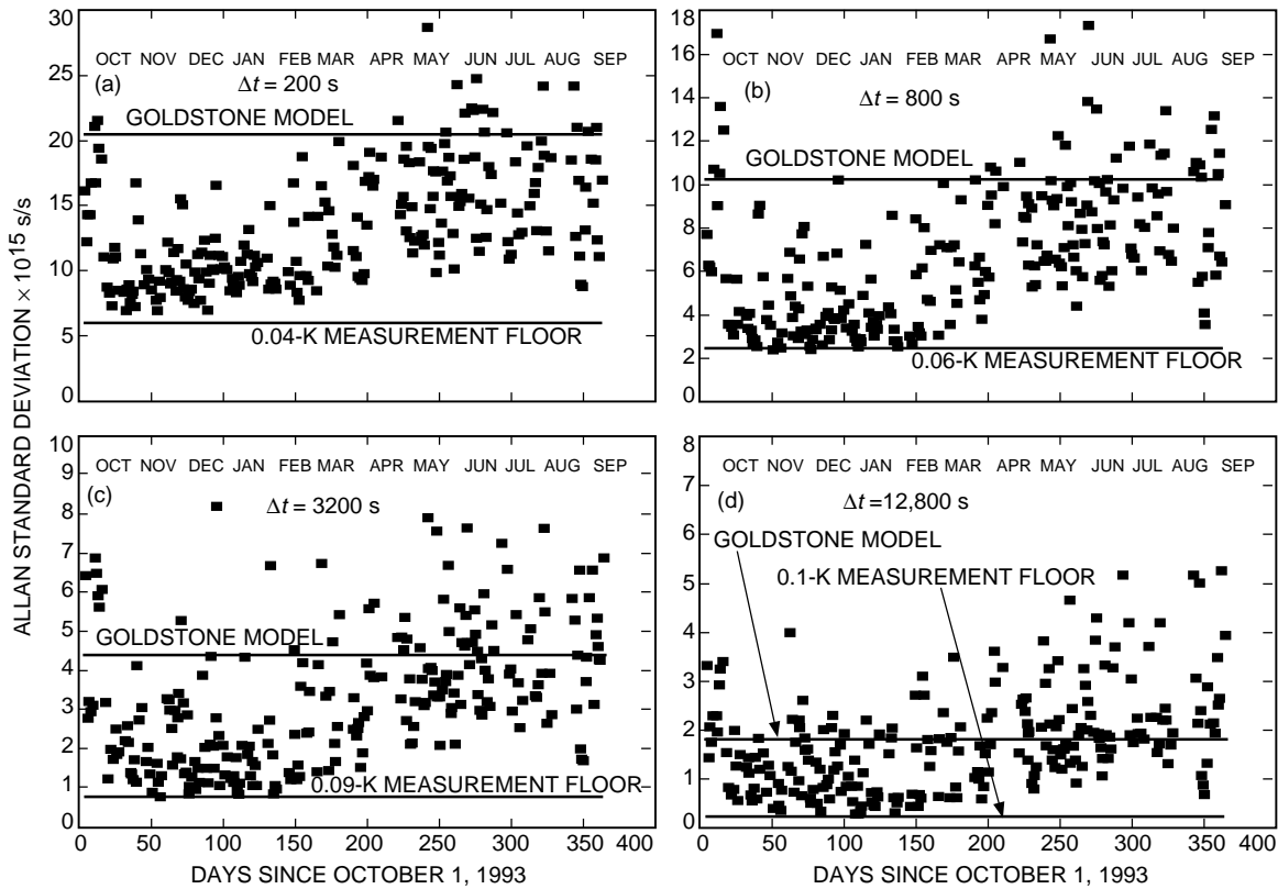
Fig. 5. WVR-derived Allan standard deviation of one-way zenith path delay at DSS 13, October 1993 through September 1994. Each data point represents the ASD calculated from ~24 hours of continuous cloud-free measurements: (a) \Delta t = 200 s, (b) \Delta t = 800 s, (c) \Delta t = 3200 s, and (d) \Delta t = 12,800 s.
