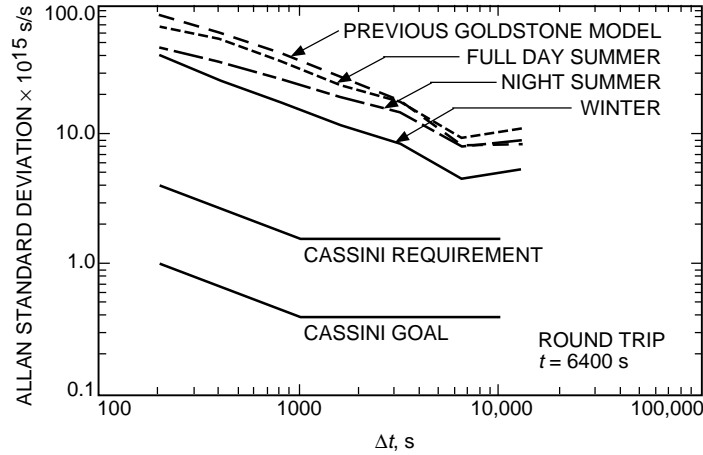
Fig. 7. Comparison of modeled and WVR-measured two-way Allan standard deviation for Goldstone at 20-deg elevation with Cassini Gravitational Wave Experiment requirements and goals.
