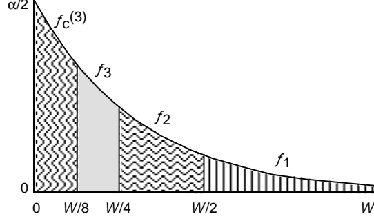
Fig. 8. Frequencies used to estimate the Laplacian parameter \alpha at the third bit layer.
