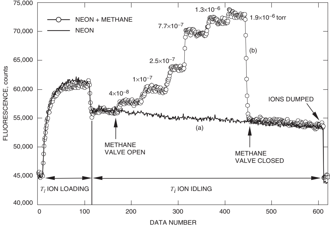
Fig. 4. Observed fluorescence when ions are loaded and dumped in a neon buffer gas environment with P_{\text{Ne}} = 3 \times 10^{-5} torr (curve a) and with step changes of partial pressure of methane gas (curve b). The step increases in the fluorescence are interpreted as relaxation of ^{199}\text{Hg} ion clock states by collisions with methane molecules.
