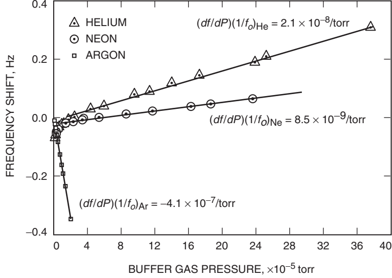
Fig. 1. Helium, neon, and argon collision shifts in the small linear ion trap. Note the effect of ion heating at low buffer gas pressures.
