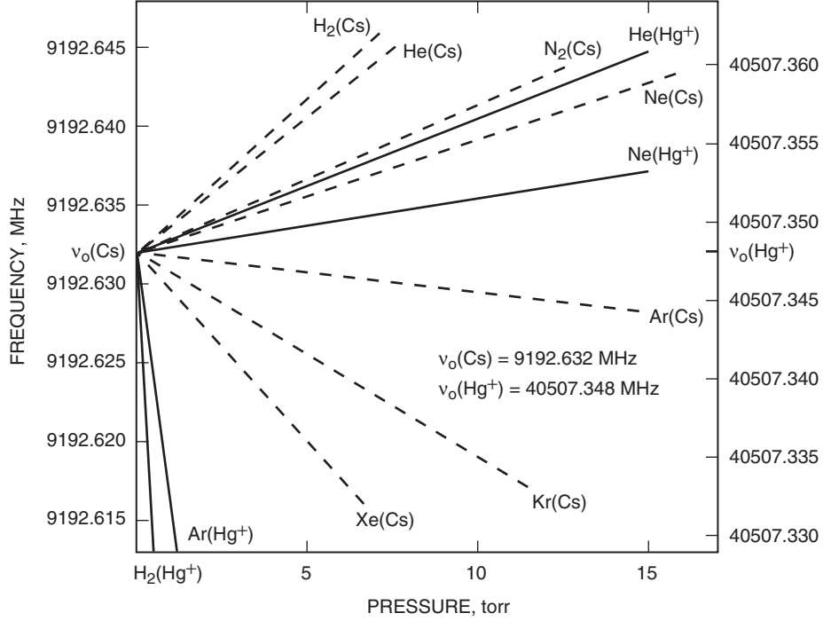
Fig. 5. Comparison of frequency shifts due to various buffer gases and residual gases for neutral cesium (Cs) atoms and mercury (Hg) ions.
