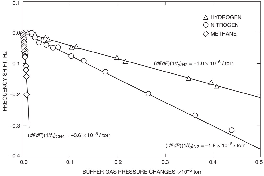
Fig. 2. Hydrogen, nitrogen, and methane gas collision shifts in the small linear ion trap. The effect of second-order Doppler shift at low pressure is not observed due to the presence of 3 \times 10^{-5} torr of neon buffer gas.
