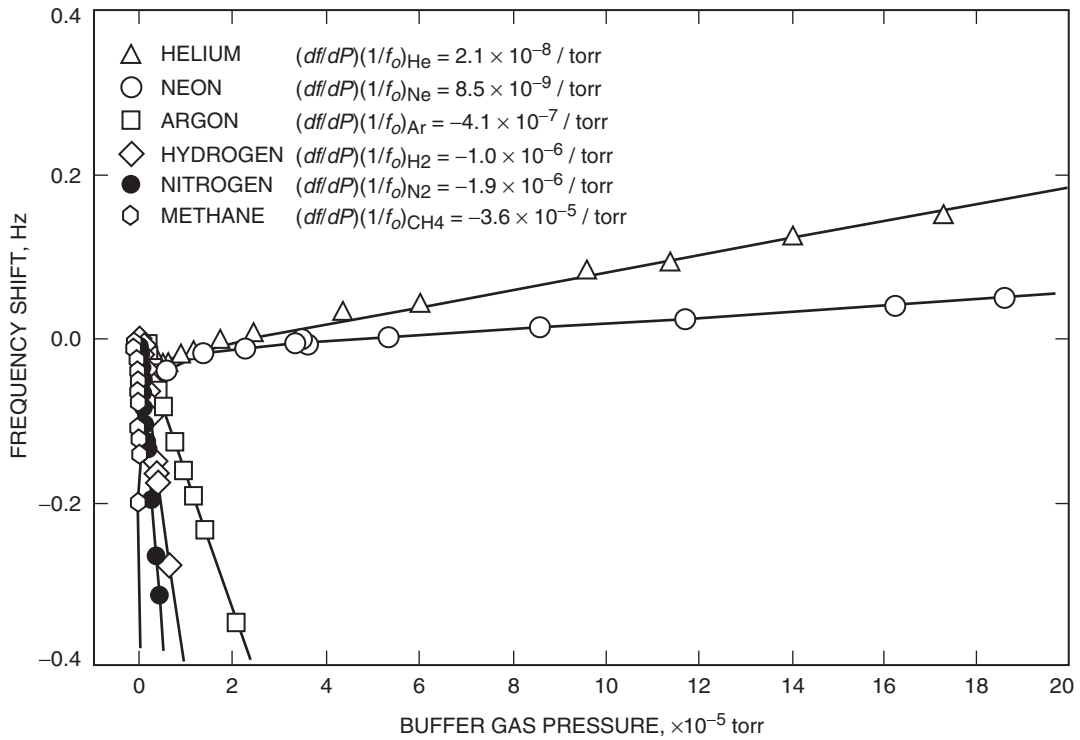
Fig. 3. Combined collision shift data with inert buffer gases and the molecular gases.
