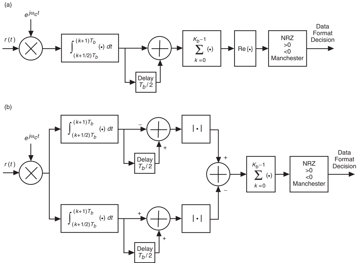
Fig. 4. Reduced-complexity noncoherent data format classifiers for BPSK modulation: (a) low SNR and (b) high SNR.
