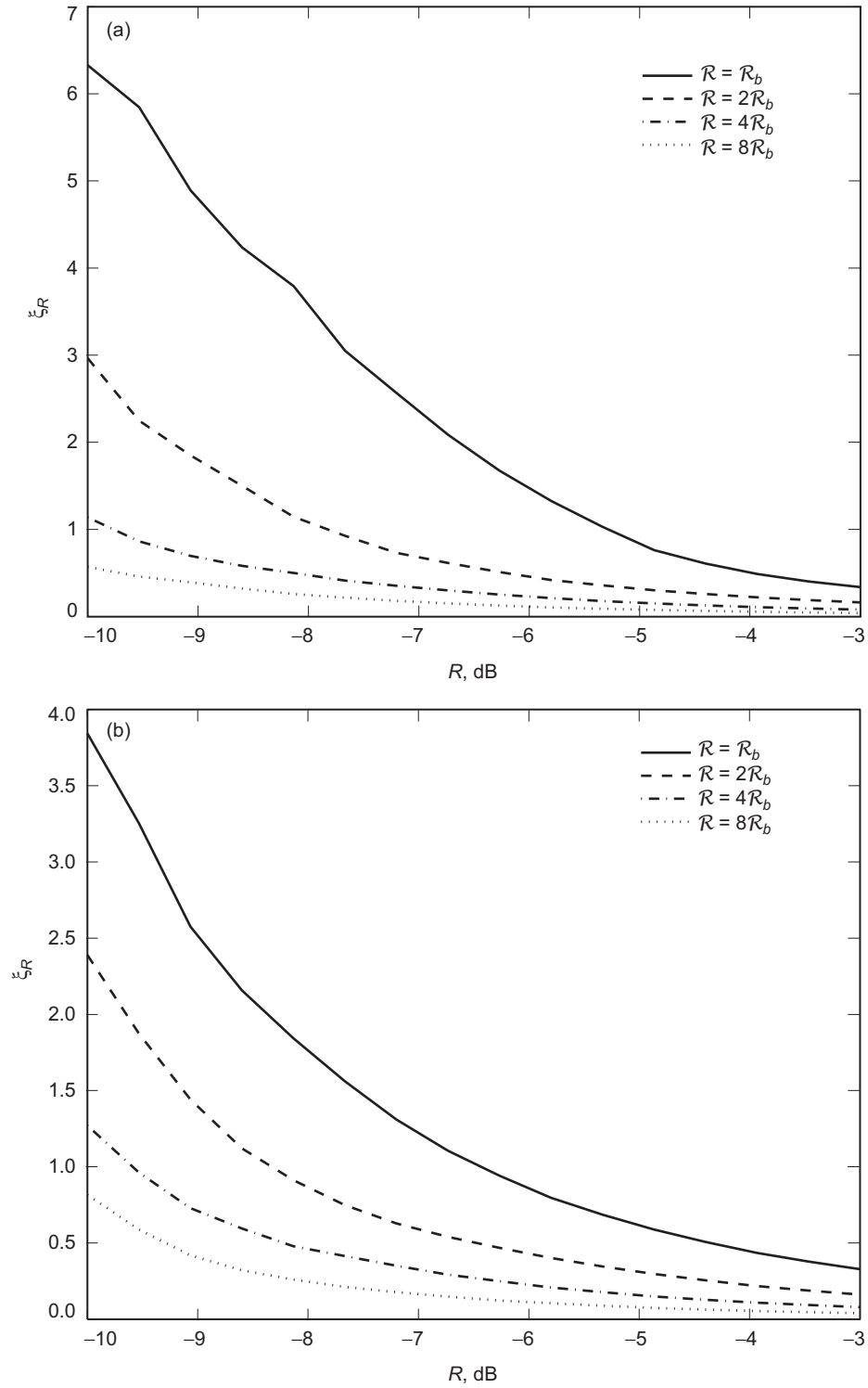
Fig. 9. Mean-squared SNR decibel estimation error as a function of the true SNR using the algorithms of (a) Section IV.B and (b) Section IV.C.
