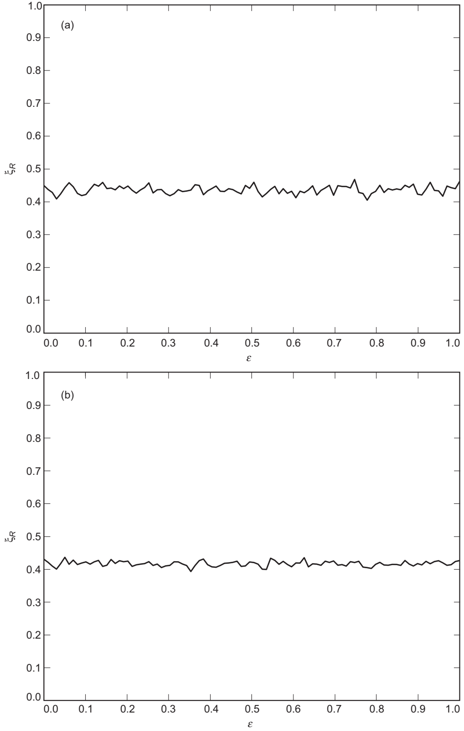
Fig. 15. Mean-squared SNR decibel estimation error as a function of the jitter using the algorithms of (a) Section IV.B and (b) Section IV.C. (The true data rate is \mathcal{R} = 2\hat{\mathcal{R}}_{b^*} )
