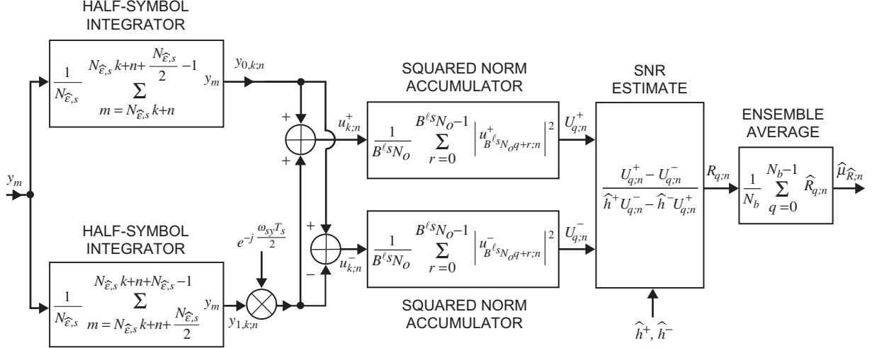
Fig. 5. Digital implementation of the SSME-based data-rate estimation system that accounts for a quantized symbol-timing error and ensemble averaging of the observed SNRs.
