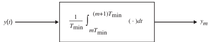
Fig. 4. System to finely integrate and sample the continuous-time signal y(t) to obtain the high-rate discrete-time signal y_m .
