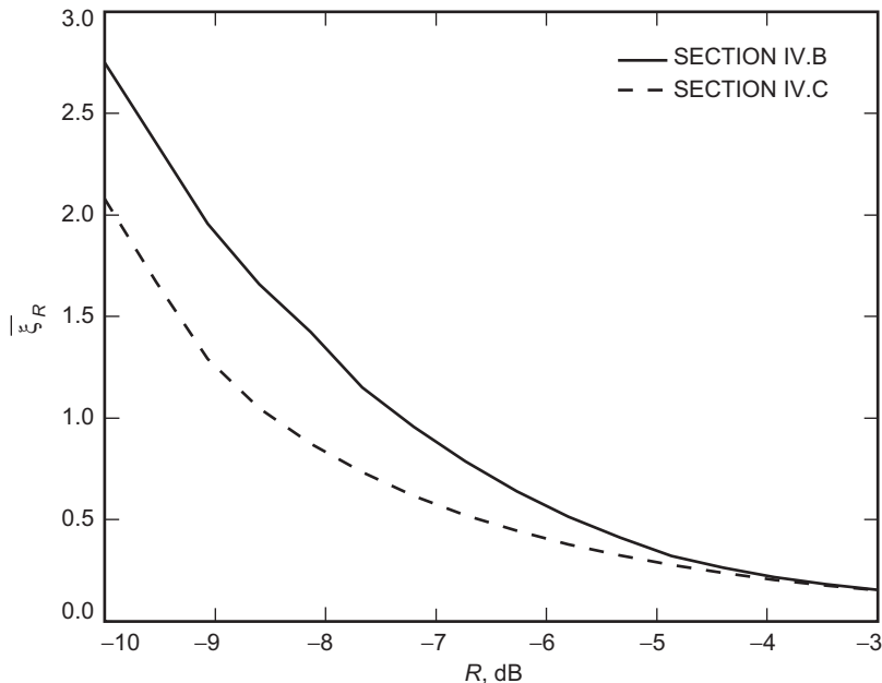
Fig. 10. Average mean-squared SNR decibel estimation error as a function of the true SNR for the algorithms of Sections IV.B and IV.C.
