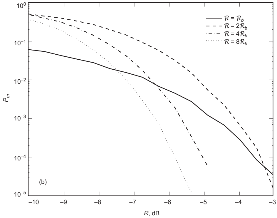
Fig. 7. Probability of data rate misclassification as a function of SNR using the algorithms of (a) Section IV.B and (b) Section IV.C.
