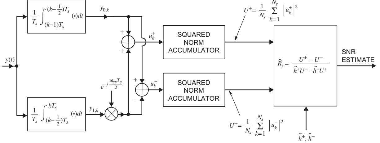
Fig. 1. SSME for a rectangular NRZ pulse shape.
