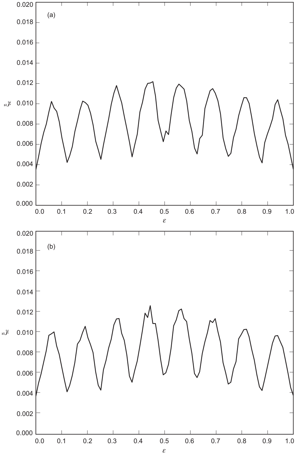
Fig. 16. Mean-squared minimum-distance symbol-timing estimation error as a function of the jitter using the algorithms of (a) Section IV.B and (b) Section IV.C. (The true data rate is \mathcal{R} = 2\mathcal{R}_b .)
