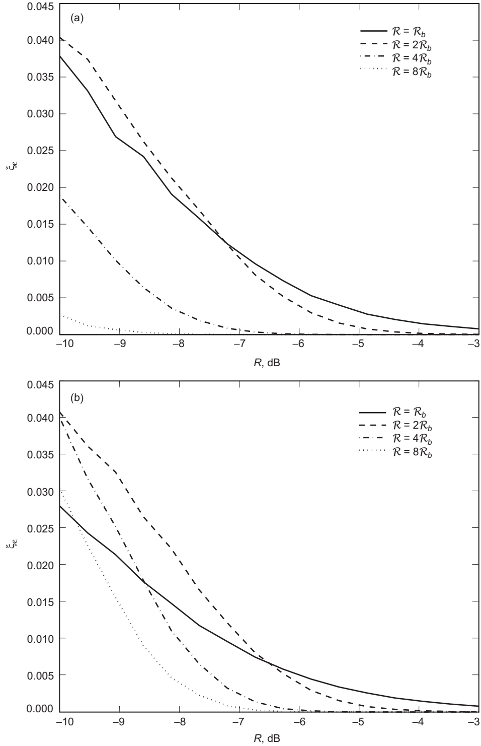
Fig. 11. Mean-squared minimum distance symbol-timing estimation error as a function of SNR using the algorithms of (a) Section IV.B and (b) Section IV.C.
