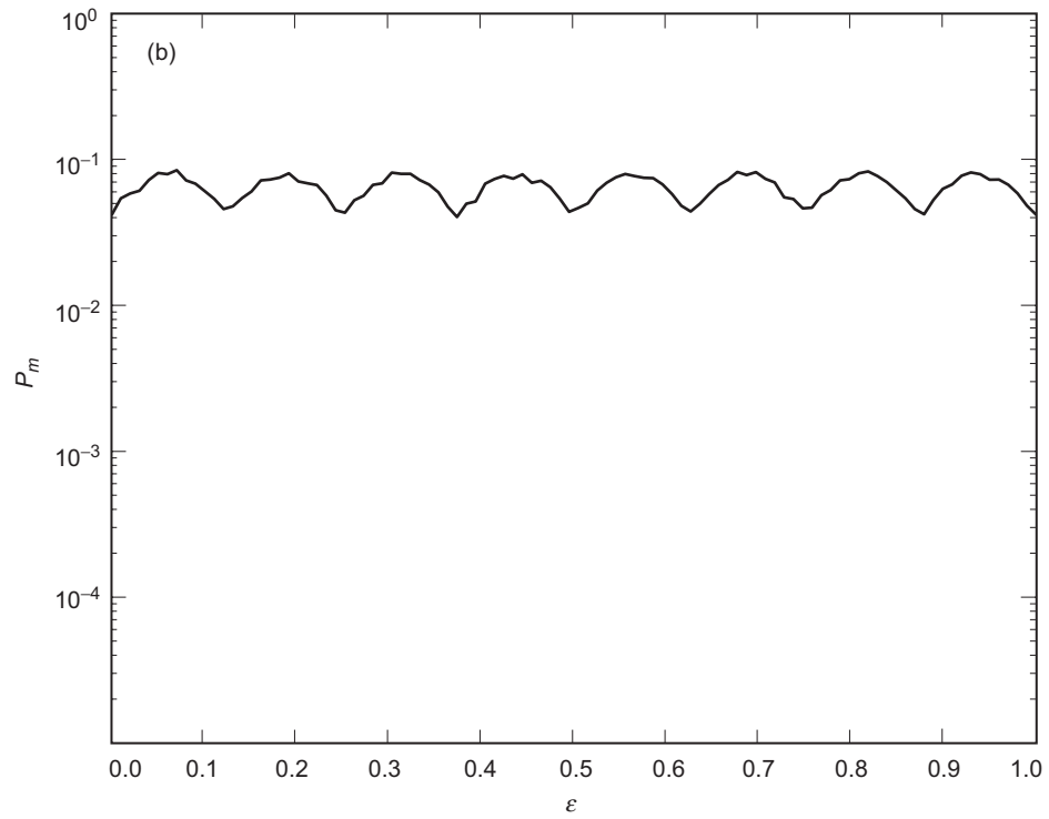
Fig. 13. Probability of data-rate misclassification as a function of the jitter using the algorithms of (a) Section IV.B and (b) Section IV.C. (The true data rate is \mathcal{R} = 2\mathcal{R}_{b,\nu} )
