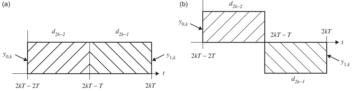
Fig. 2. Signal component of the I&D outputs y_{0,k} and y_{1,k} when the SSME assumed data rate is half of the true data rate for the case of (a) identical and (b) different adjacent data symbols.
