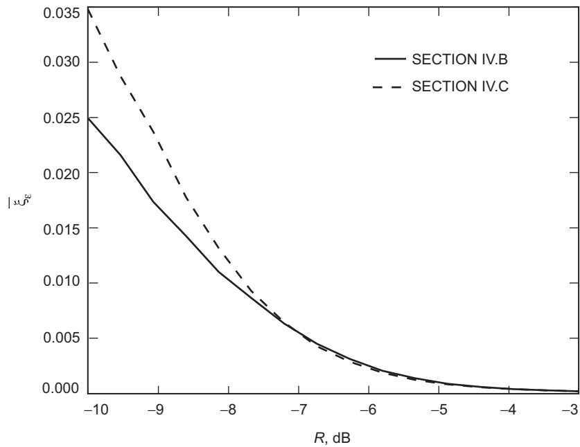
Fig. 12. Average mean-squared minimum distance symbol-timing estimation error as a function of SNR for the algorithms of Sections IV.B and IV.C.
