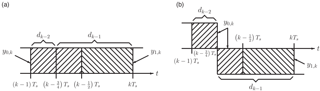
Fig. 3. Signal component of the I&D outputs y_{0,k} and y_{1,k} when the symbol-timing error is \epsilon = 1/4 for the case of (a) identical and (b) different adjacent data symbols.
