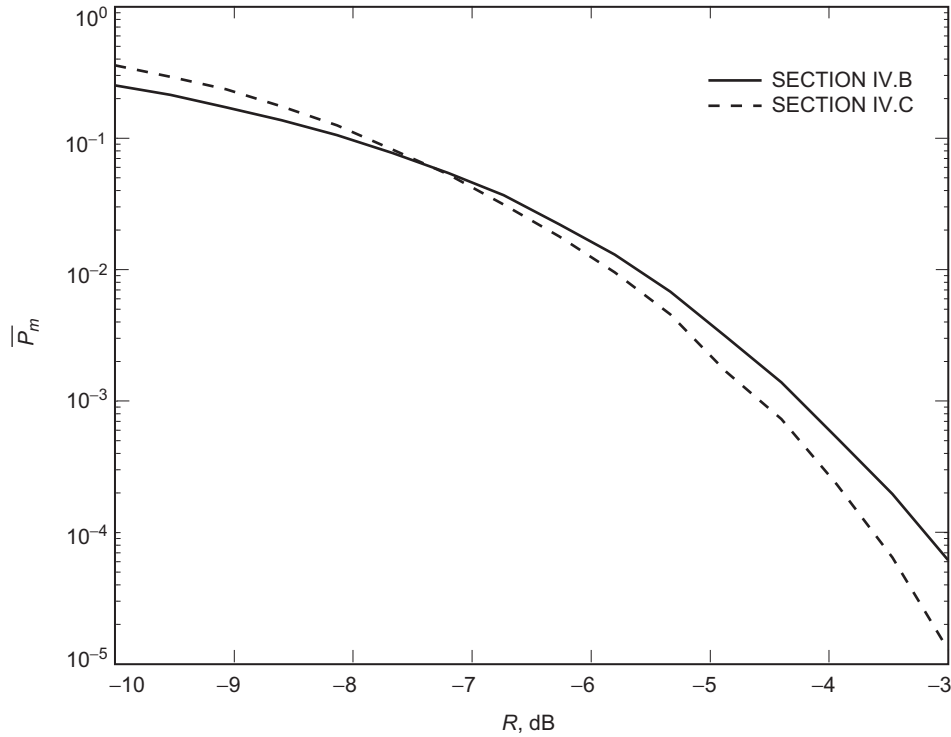
Fig. 8. Average probability of misclassification as a function of SNR for the algorithms of Sections IV.B and IV.C.
