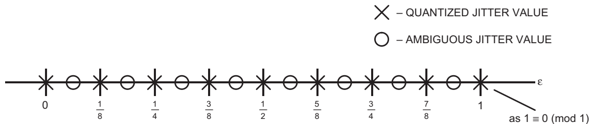
Fig. 14. Example showing the quantized symbol-timing error values for N_{\epsilon,s} = 8 along with the ambiguous jitter values.
