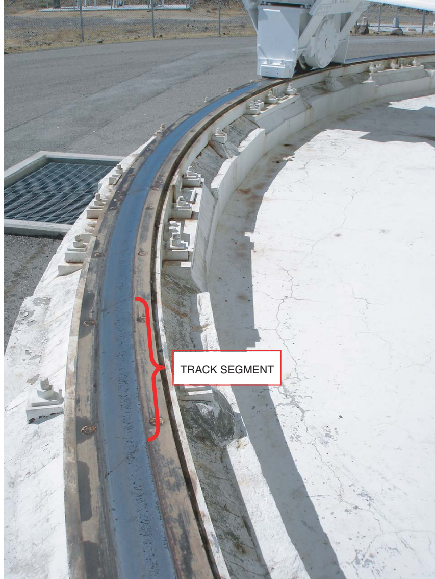
Fig. 2. The DSS 25 antenna's azimuth track.
