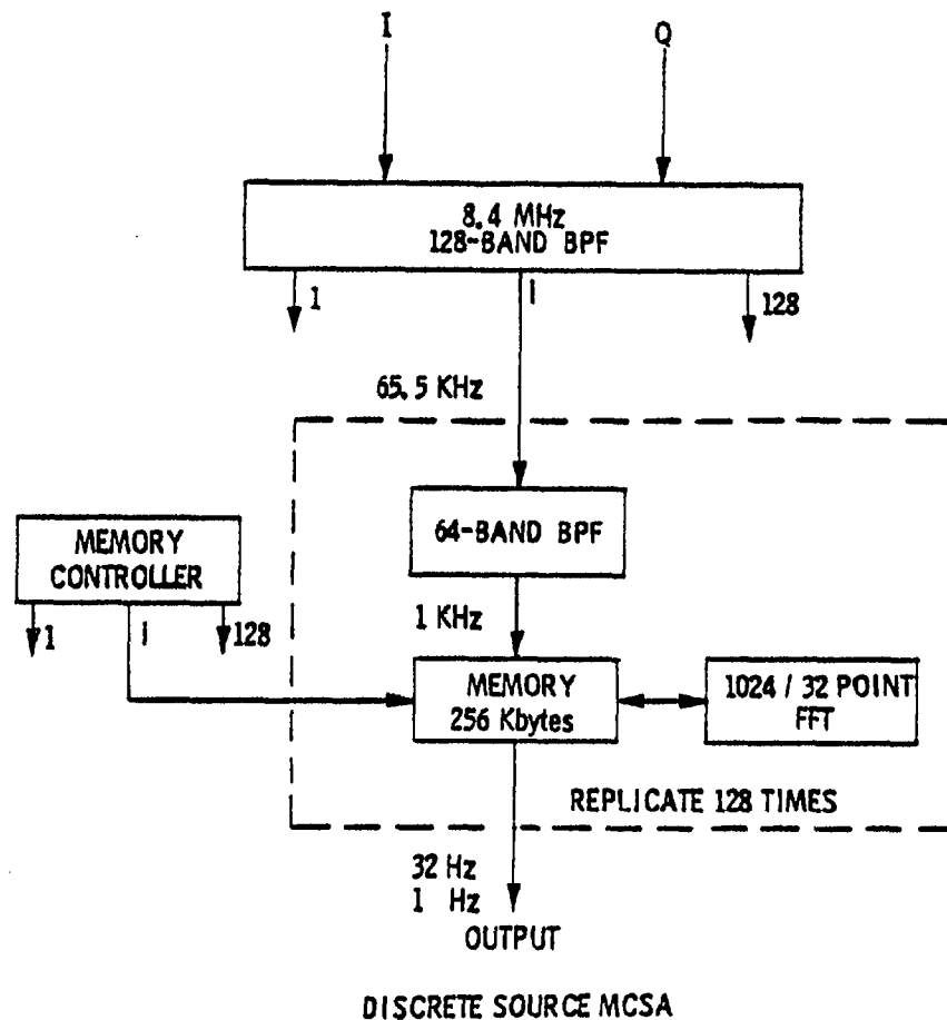
Fig. 4. A schematic block diagram of the multichannel spectrum analyzer designed for the discrete source survey. It is designed to cover a 8.4-MHz instantaneous bandpass at 1-Hz resolution
