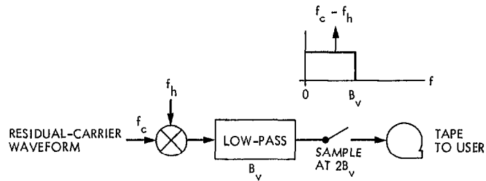
Fig. 1. Conceptual model of residual-carrier, open-loop receiver
