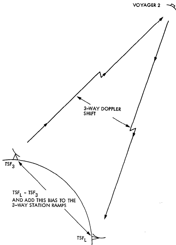
Fig. 3. Voyager 2 three-way acquisition
