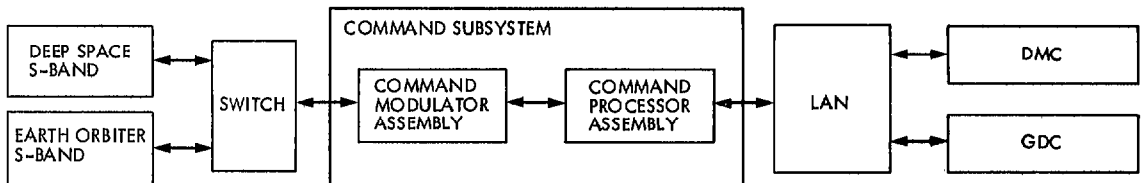
Fig. 3. Command Subsystem configurations
