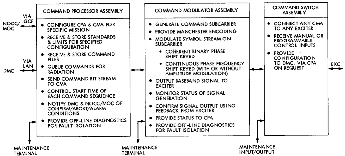
Fig. 2. Allocation of functions to assemblies
