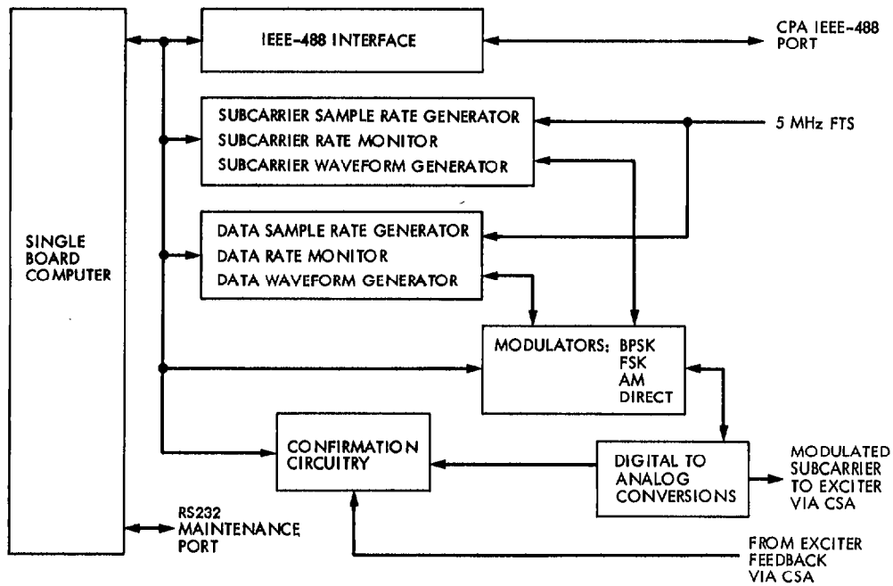
Fig. 5. Command modulator assembly, functional block diagram
