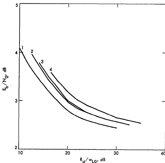
Fig. 4. Array total E_b/N_0 needed to achieve an error rate P_E = 0.005 , with carrier suppression from Fig. 2. Arrays: (1) One antenna, w_{L0} = 30 Hz; (2) 64 m - 34 m, 10 Hz; (3) 64-34-34 m, 10 Hz; (4) 64-34-34-34 m, 10 Hz. Conditions: same as Fig. 2
