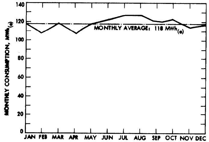
Fig. 4. Electrical consumption on a monthly basis, Venus Station
