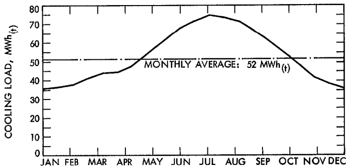
Fig. 2. Monthly cooling load of the Venus Station
