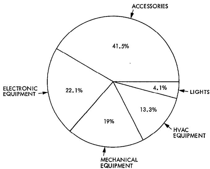
Fig. 3. Itemization of annual electrical consumption, Venus Station
