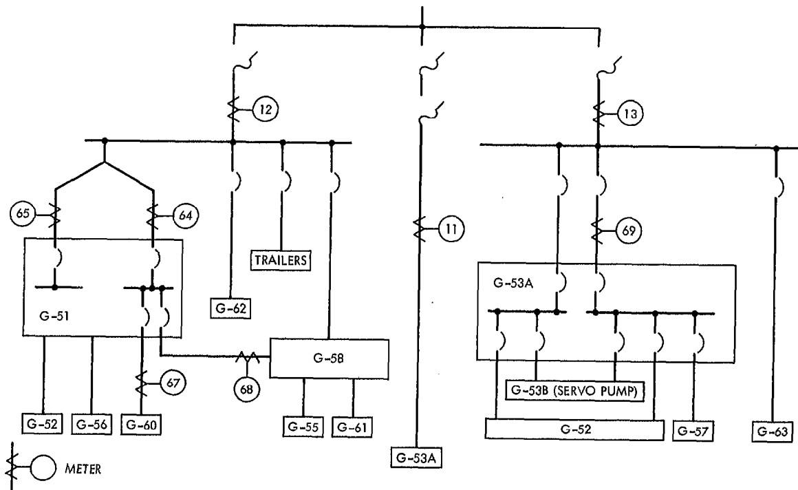
Fig. 10. Layout of watt-hour meters at Venus Station
