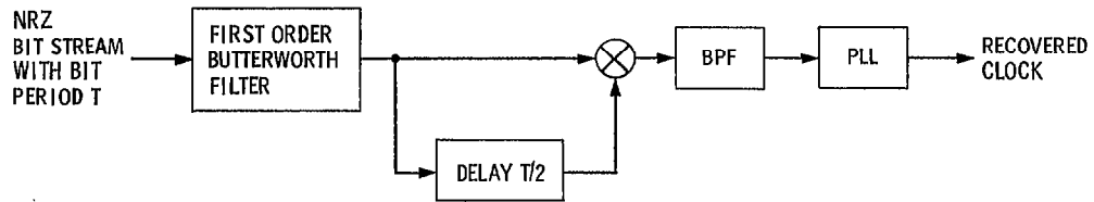
Fig. 1. Baseband delay and multiply circuit
