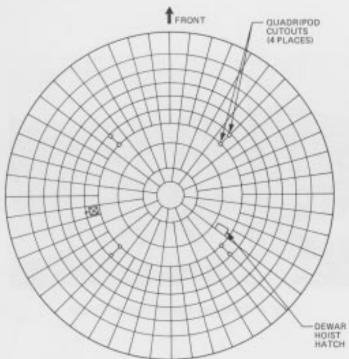
Fig. 11. Reflector panel assembly, from zenith down, DSS 15
