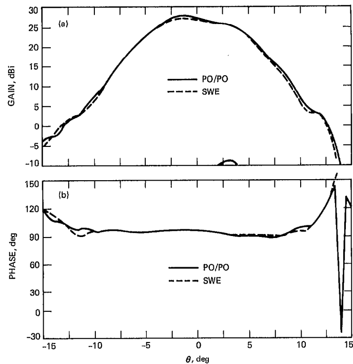
Fig. 15. PO and SWE far-field scattering from two 2.4-m paraboloids at 2.3 GHz: (a) amplitude; (b) phase
