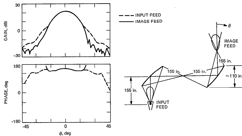
Fig. 18. GTD scattering for two 2.4-m ellipses, RCP at 8.4 GHz
