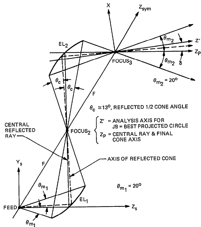
Fig. 11. Analysis geometry for ellipsoid pair ( EL_1 , EL_2 )
