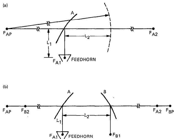
Fig. 6. Bandpass feed imaging configuration
