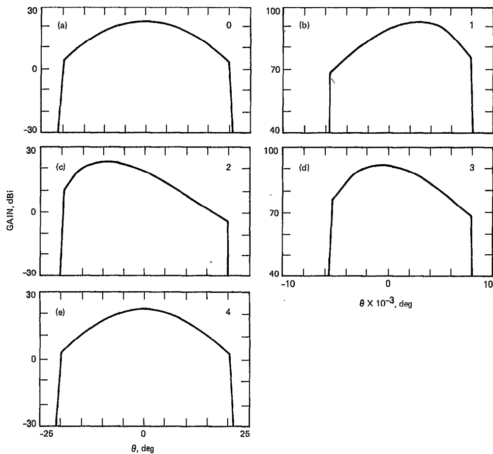
Fig. 5. Geometrical optics field reflected from each surface of a beam-waveguide system (shown in Fig. 3[a]): (a) input pattern; (b) reflected field from S_1 ; (c) reflected field from S_2 ; (d) reflected field from S_3 ; (e) reflected field from S_4 or output pattern
