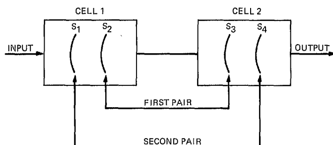
Fig. 2. Multiple curved reflector beam-waveguide system; S_i = ellipsoid, hyperboloid, or paraboloid
