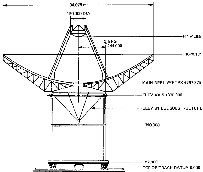
Fig. 8. 34-m H.E. existing structure
