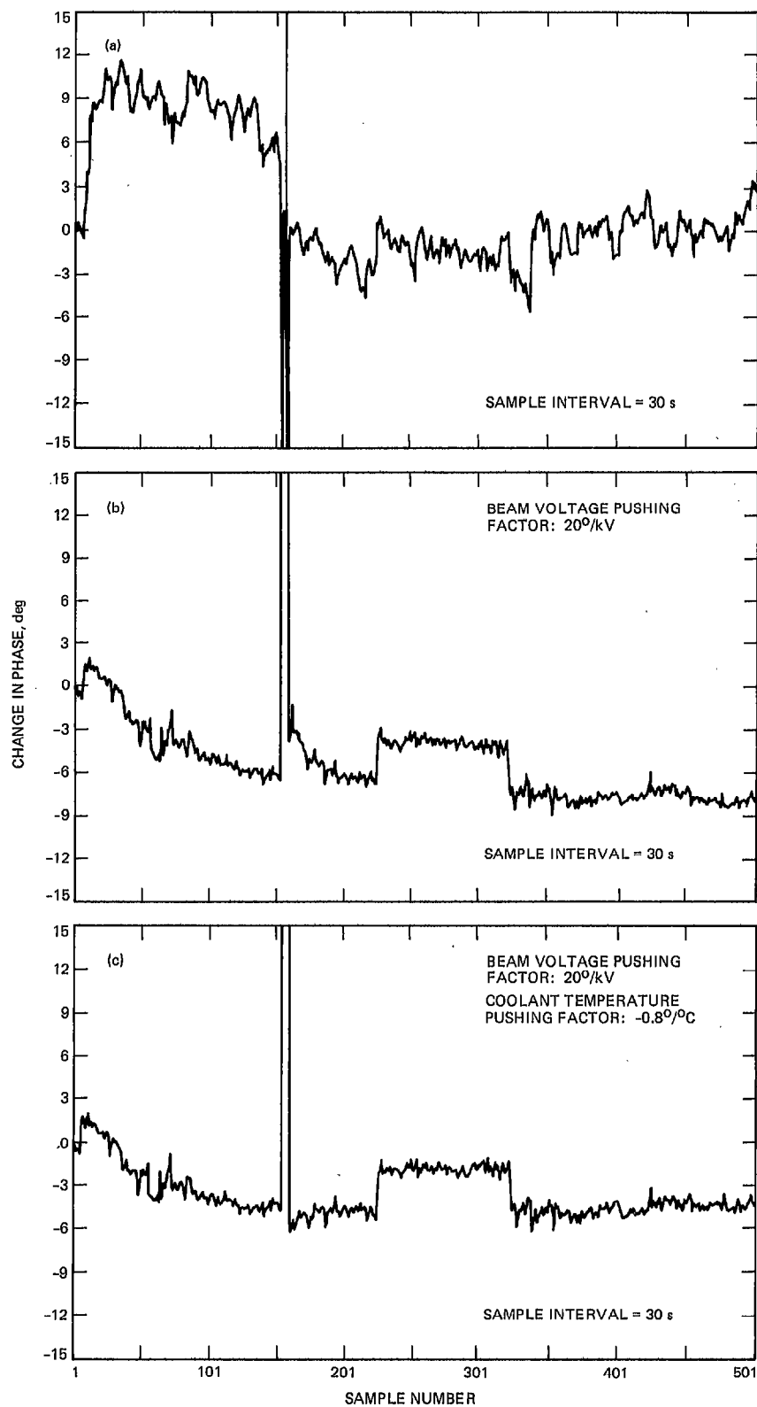
Fig. 7. Change in phase: (a) uncorrected, (b) beam voltage corrected, (c) beam voltage and temperature corrected
