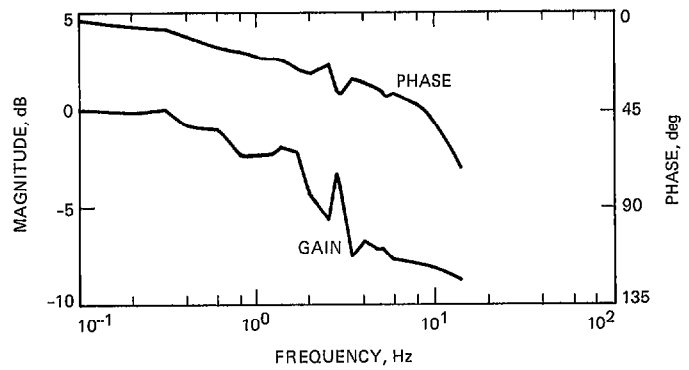
Fig. 14. Unbiased input test — elevation axis loop, EL = 88 deg
