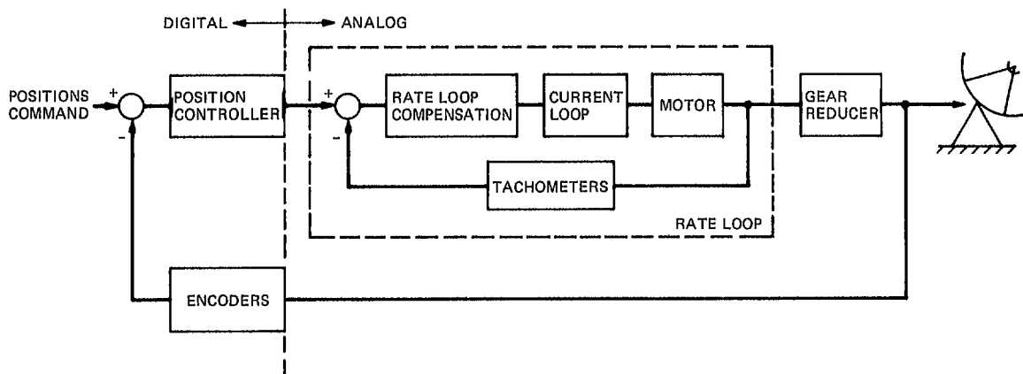
Fig. 1. Position loop
