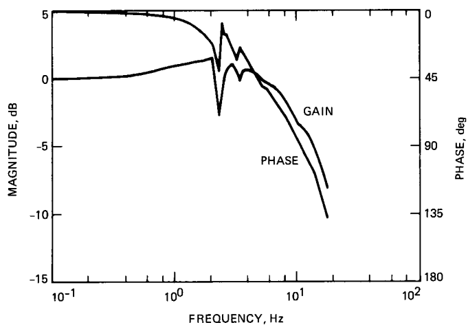
Fig. 7. Biased input test — elevation axis loop, EL = 7 deg
