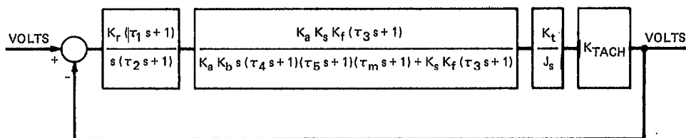
Fig. 2. Rate loop
