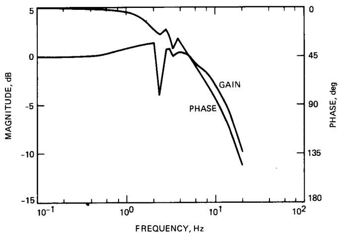
Fig. 8. Biased input test — elevation axis loop, EL = 45 deg
