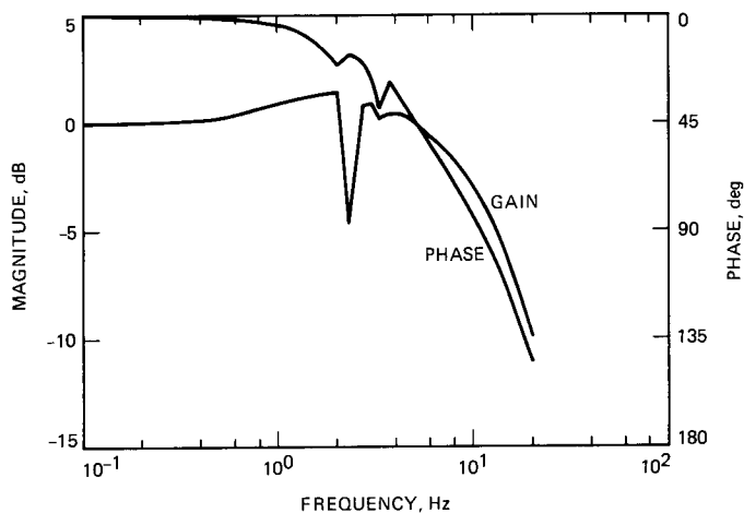
Fig. 9. Biased input test — elevation axis loop, EL = 70 deg
