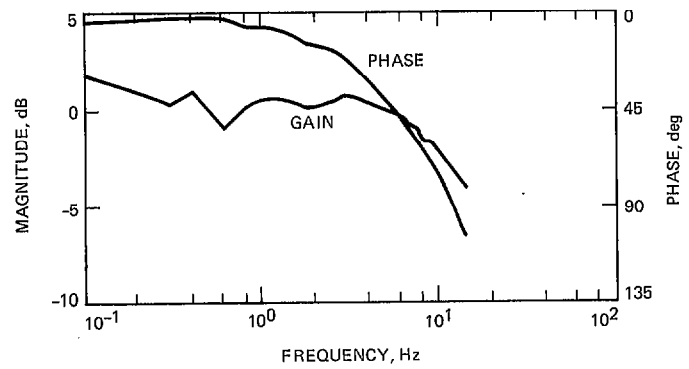
Fig. 15. Biased input test — azimuth axis loop, EL = 7 deg
