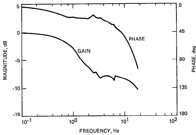
Fig. 11. Unbiased input test — elevation axis loop, EL = 7 deg
